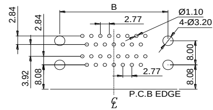
RECOMMENDED P.C.B LAYOUT FOR ALL SERIES
