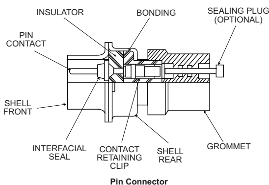
Pin Connector
