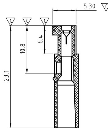
Section P-P
