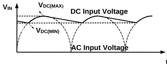
(b) V_{IN} of Full-Wave Rectifier
