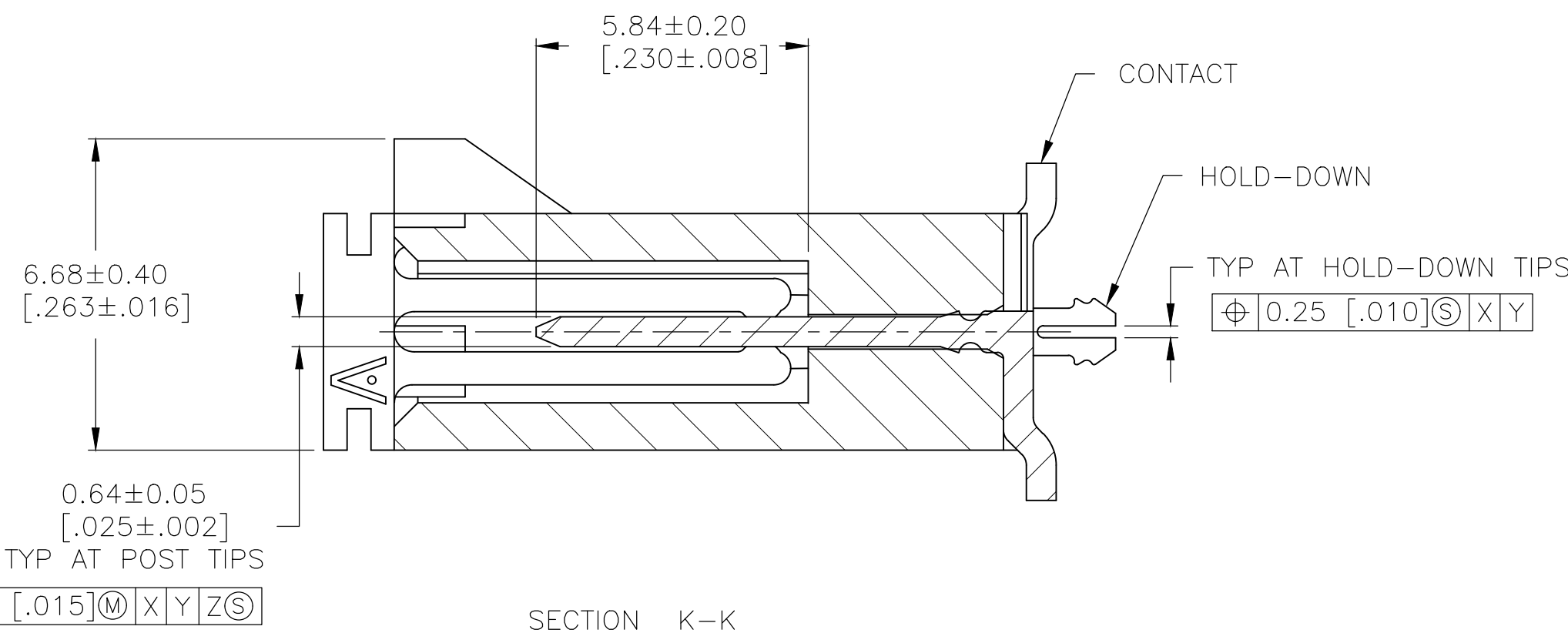
SECTION K-K
