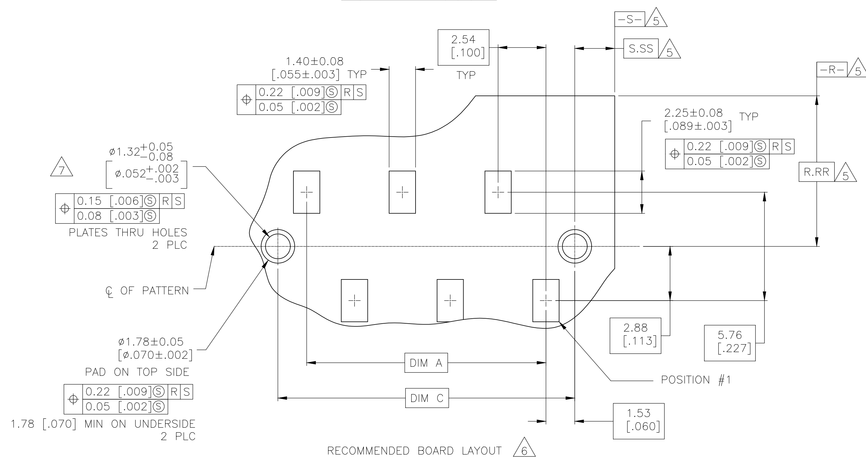
RECOMMENDED BOARD LAYOUT
