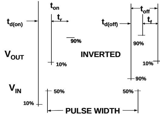
Figure 2: Switching Waveforms
