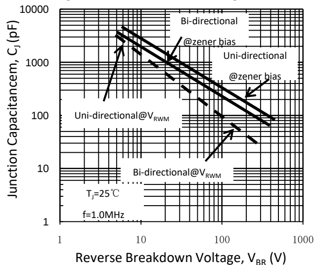
Fig. 6-Typical Junction Capacitance
