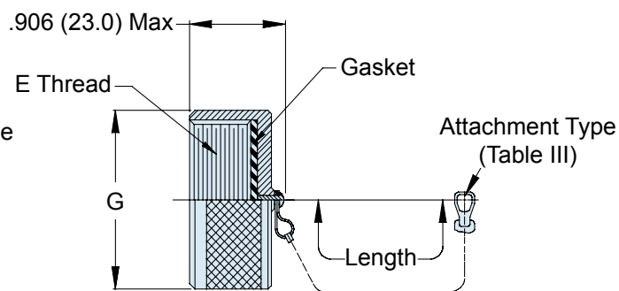
660-024 Receptacle Cover
