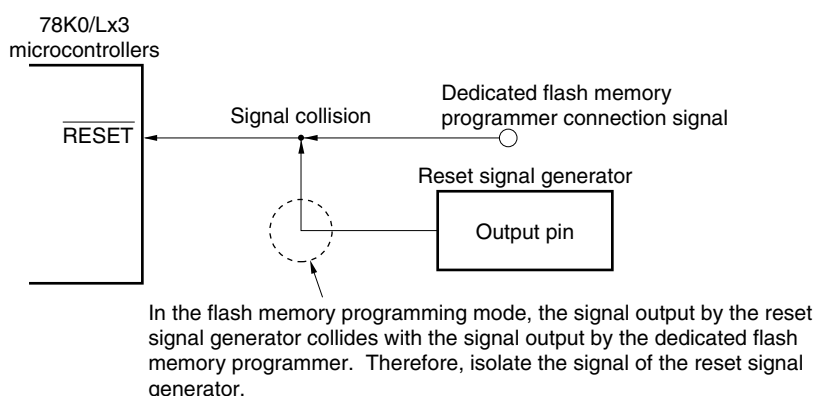
Figure 28-9. Signal Collision (RESET Pin)
