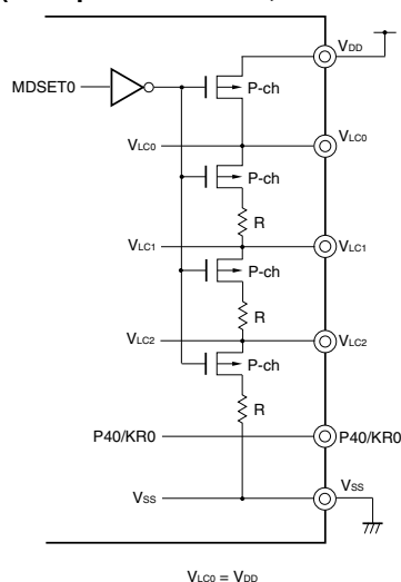
(a) 1/3 bias method and static display mode (MDSET1, MDSET0 = 0, 1) (example of V_{DD} = 5\text{ V} , V_{LC0} = 5\text{ V} )
