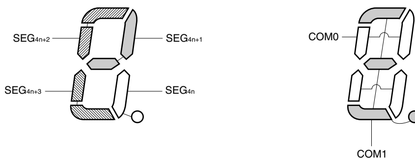
Figure 18-23. Two-Time-Slice LCD Display Pattern and Electrode Connections
