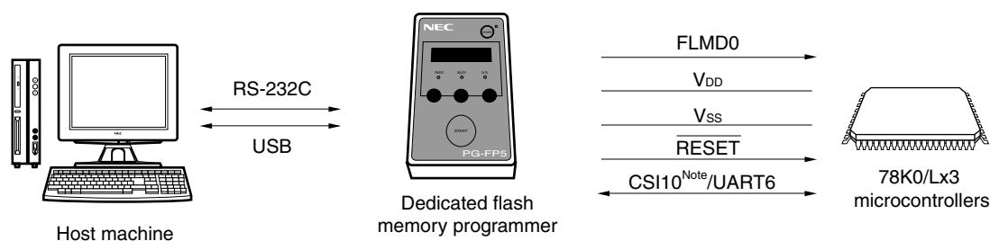
Figure 28-3. Environment for Writing Program to Flash Memory
