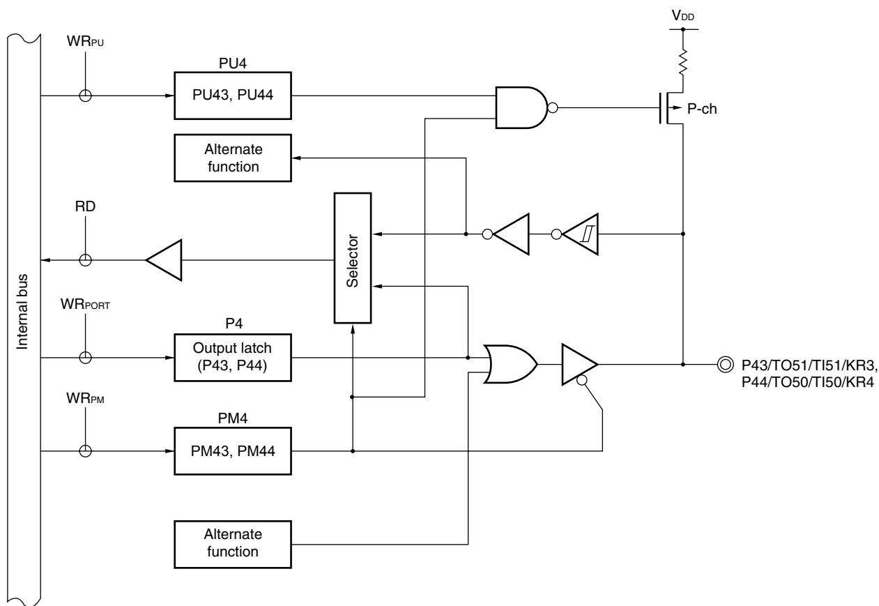
Figure 4-13. Block Diagram of P43 and P44
