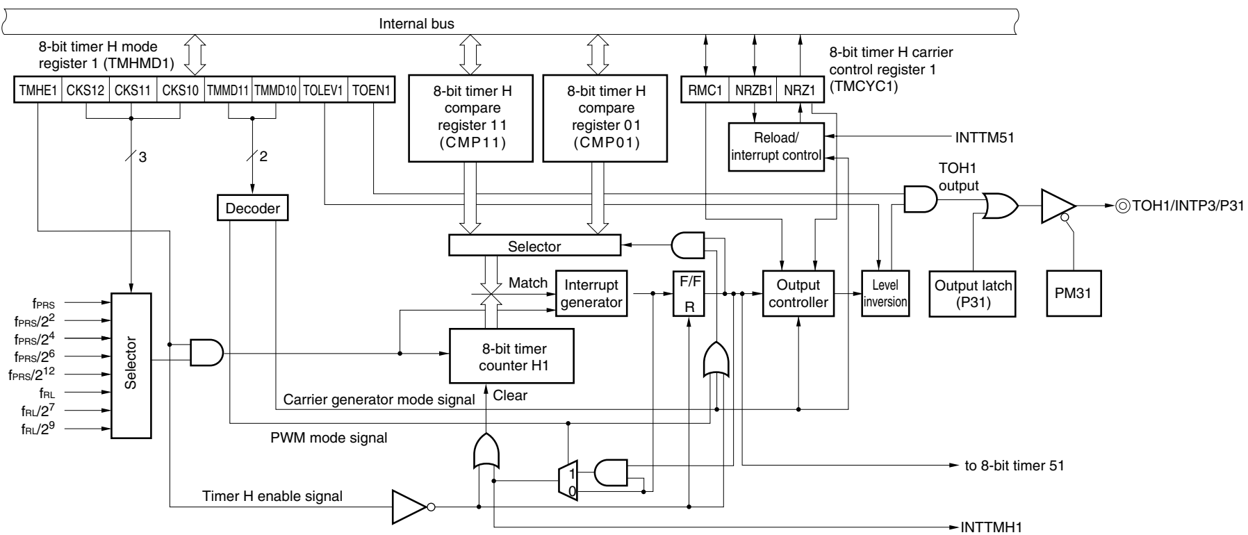
Figure 8-2. Block Diagram of 8-Bit Timer H1
