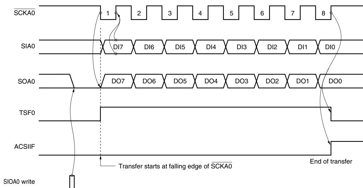
Figure 17-11. 3-Wire Serial I/O Mode Timing
