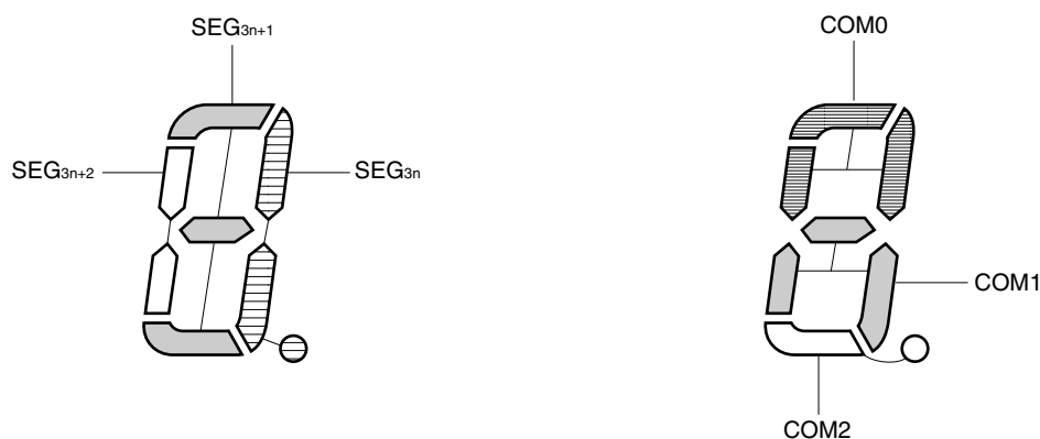
Figure 18-26. Three-Time-Slice LCD Display Pattern and Electrode Connections
