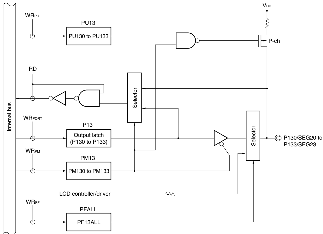
Figure 4-23. Block Diagram of P130 to P133
