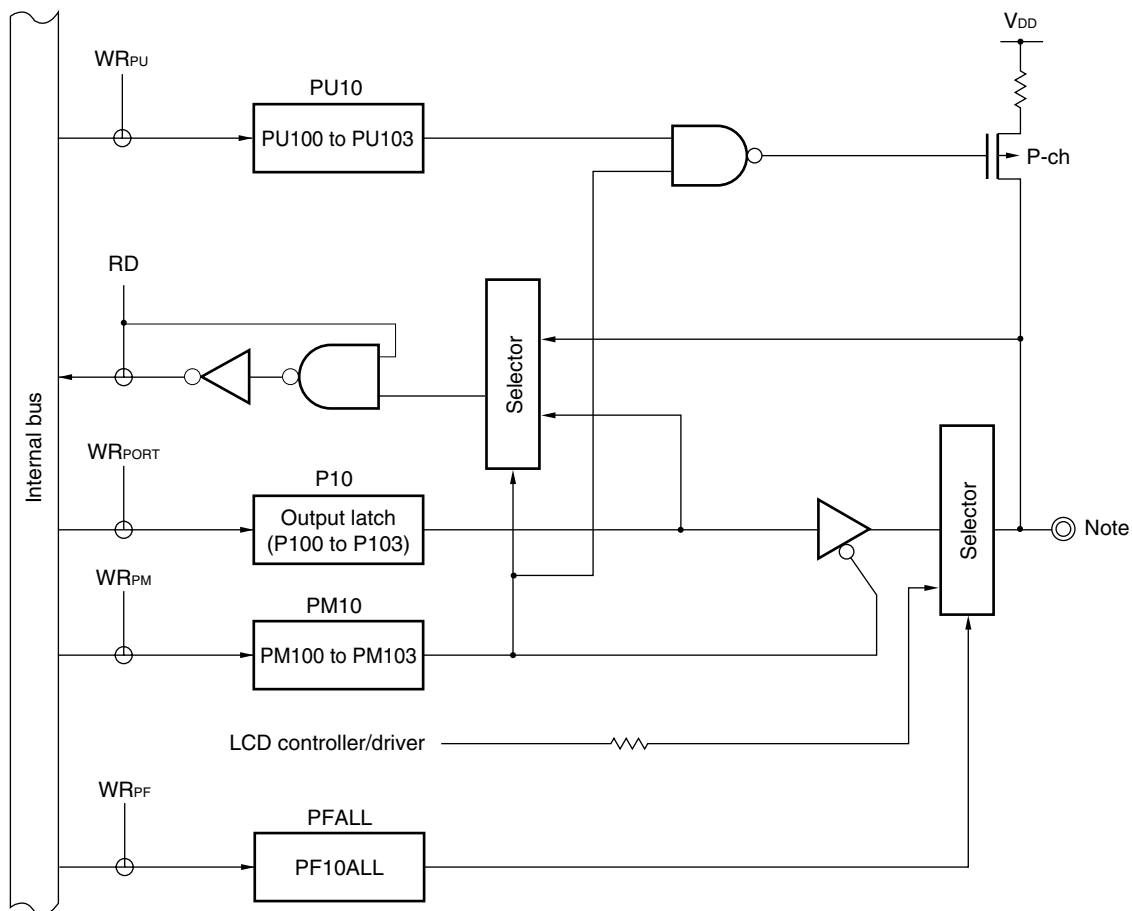
Figure 4-16. Block Diagram of P100 to P103
