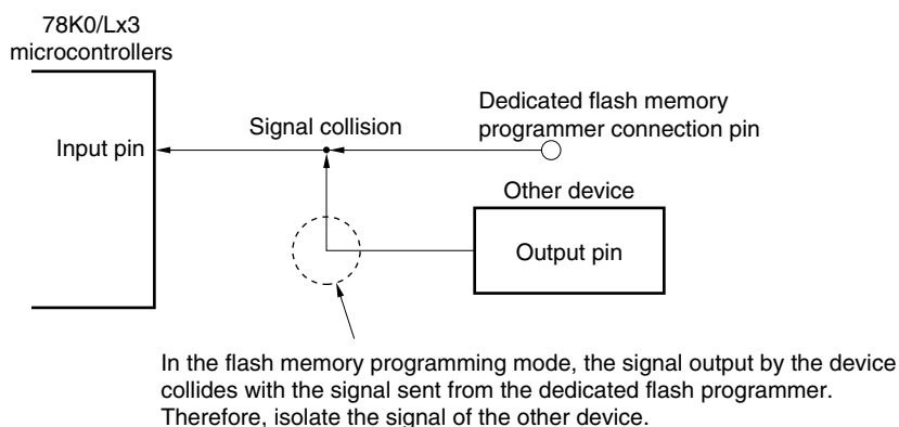
Figure 28-7. Signal Collision (Input Pin of Serial Interface)
