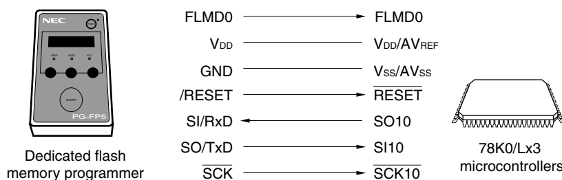
Figure 28-4. Communication with Dedicated Flash memory programmer (CSI10)
