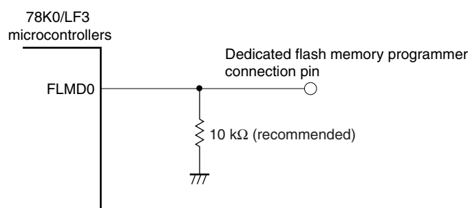
Figure 28-6. FLMD0 Pin Connection Example
