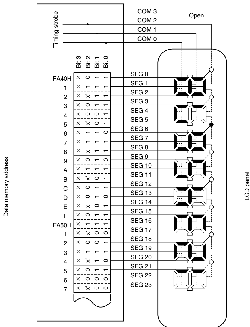
Figure 18-27. Example of Connecting Three-Time-Slice LCD Panel
