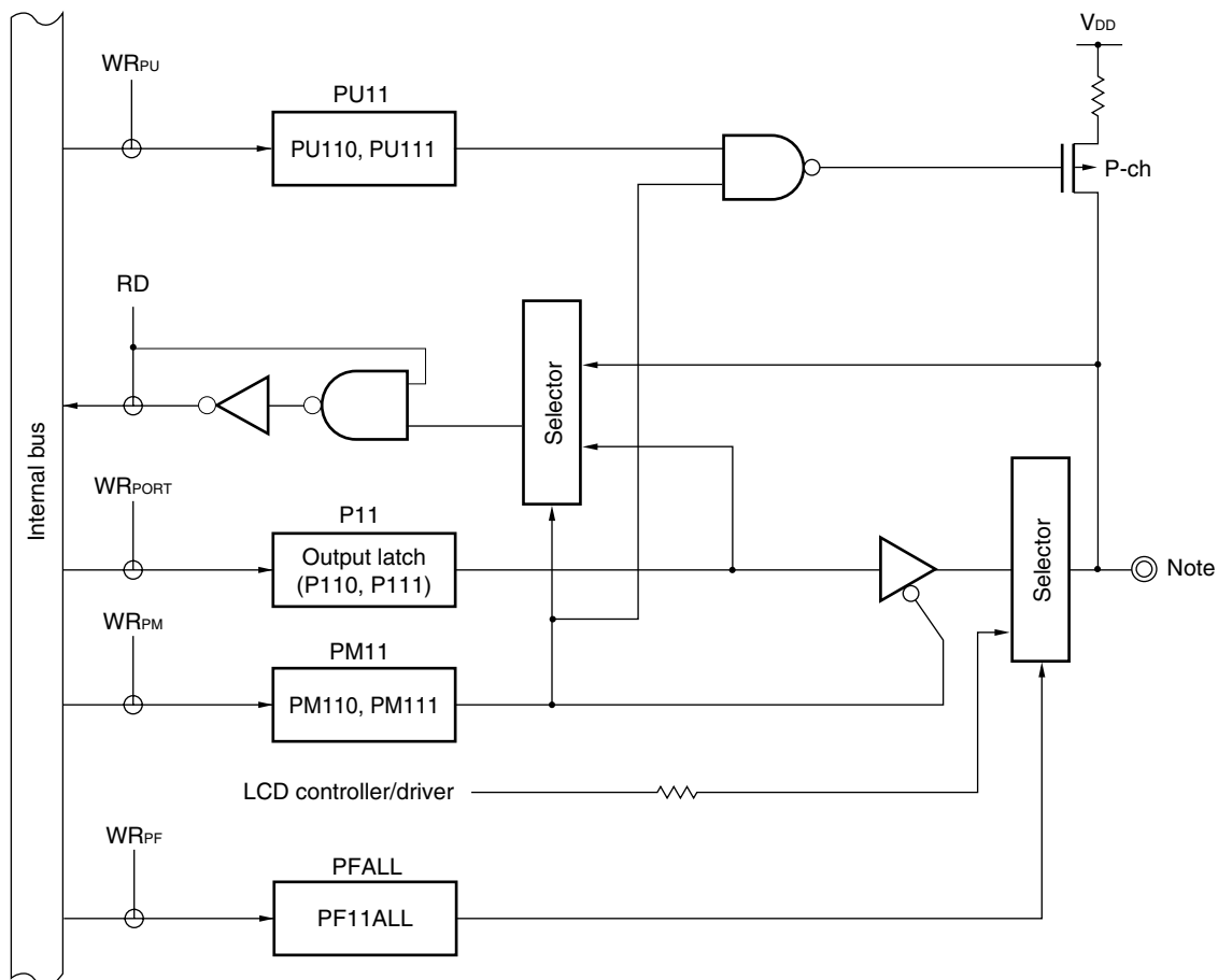
Figure 4-17. Block Diagram of P110 and P111
