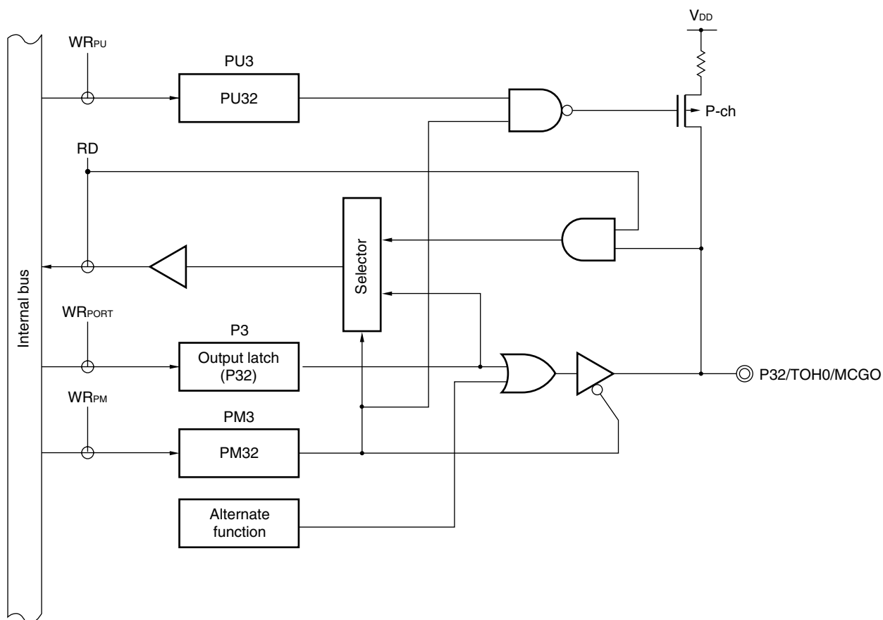
Figure 4-10. Block Diagram of P32
