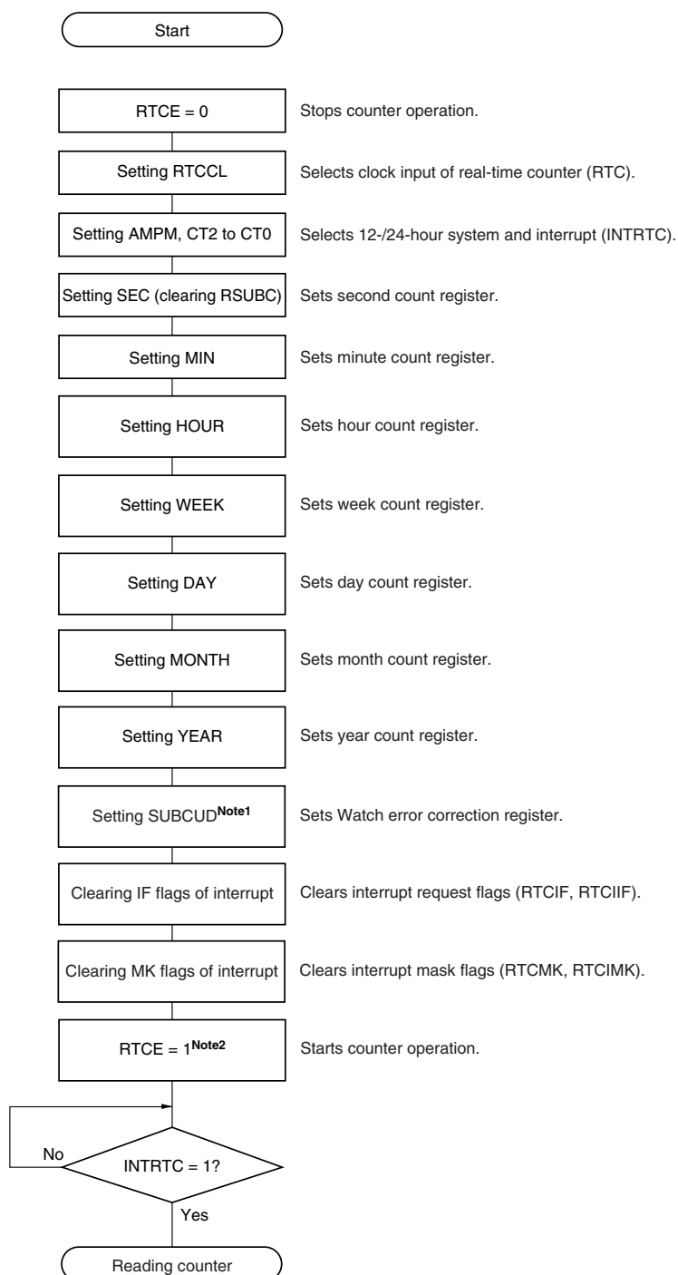
Figure 9-19. Procedure for Starting Operation of Real-Time Counter
