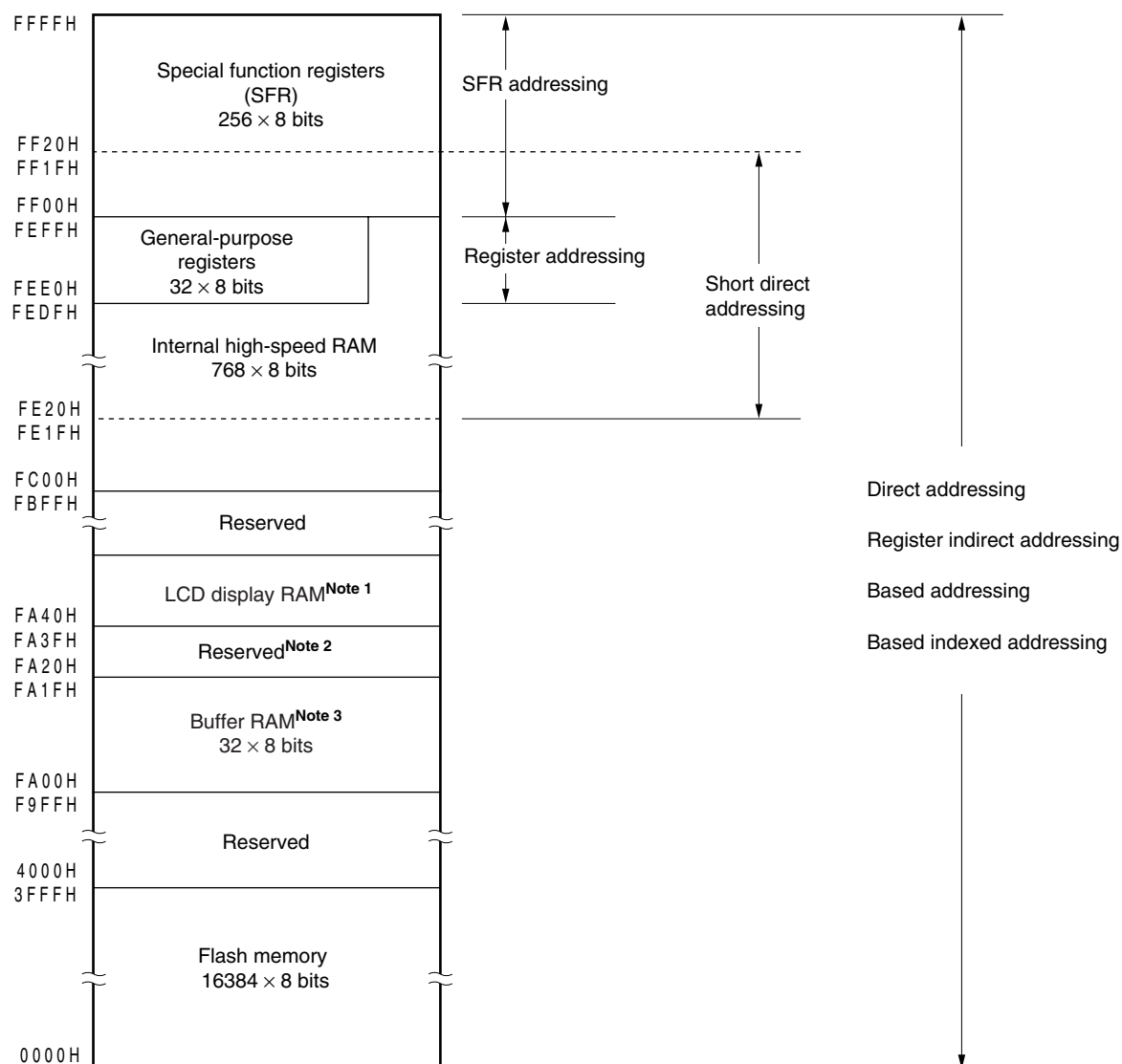
Figure 3-8. Correspondence Between Data Memory and Addressing ( \mu PD78F04x1)
