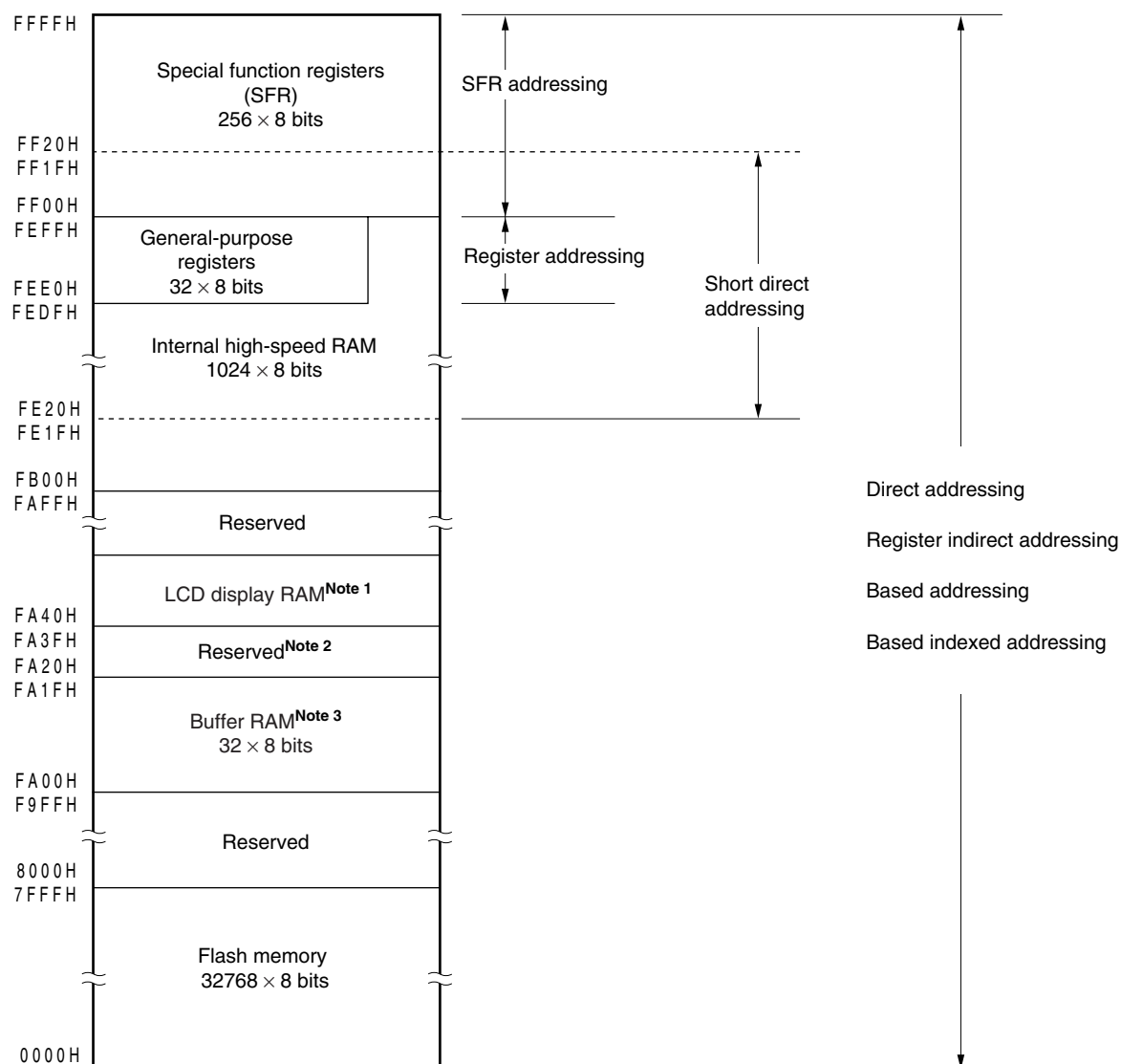
Figure 3-10. Correspondence Between Data Memory and Addressing ( \mu PD78F04x3)
