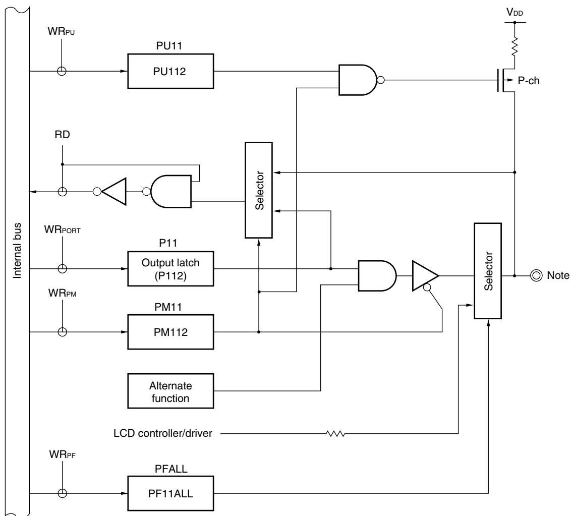
Figure 4-18. Block Diagram of P112
