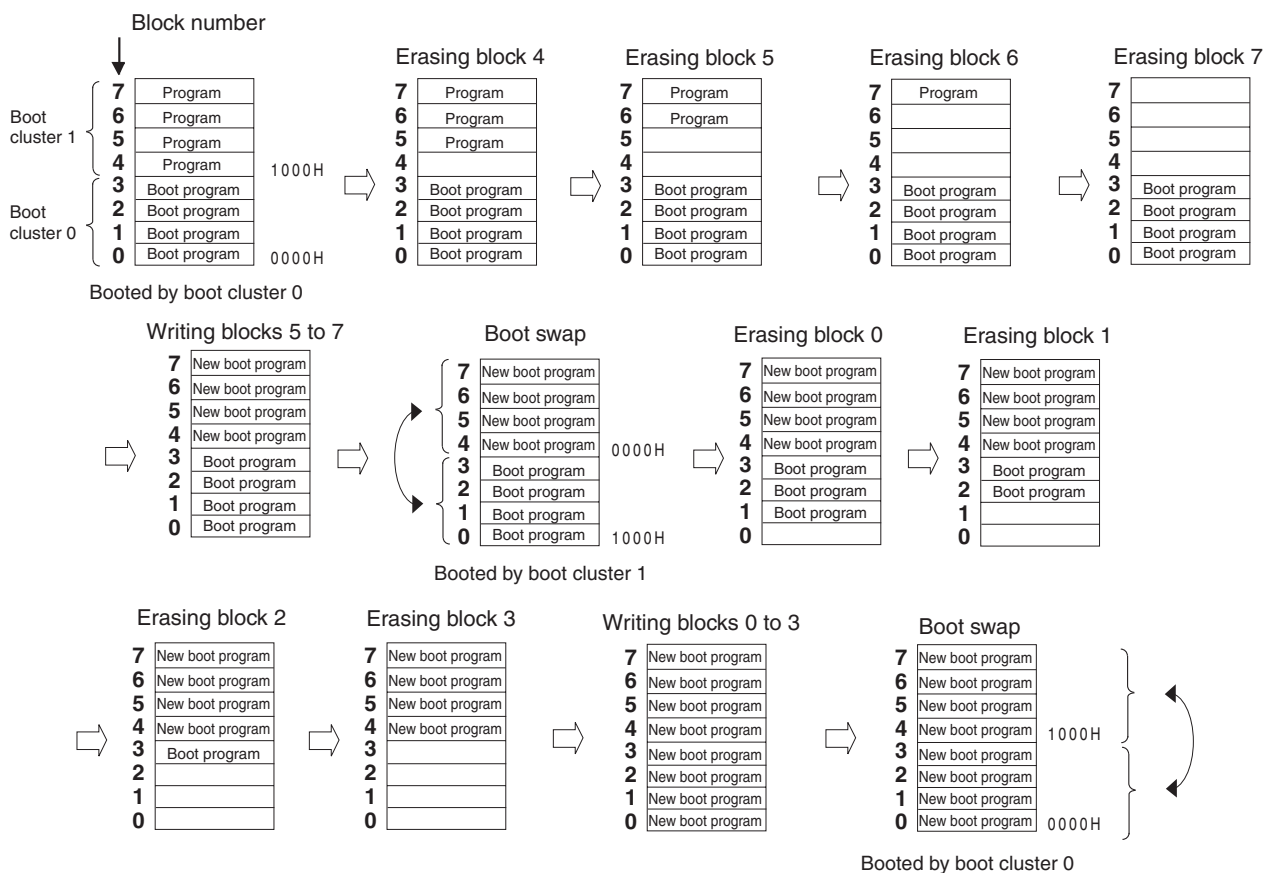
Figure 28-16. Example of Executing Boot Swapping
