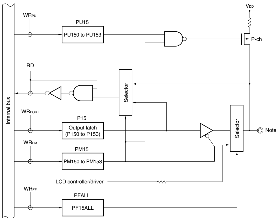
Figure 4-25. Block Diagram of P150 and P153
