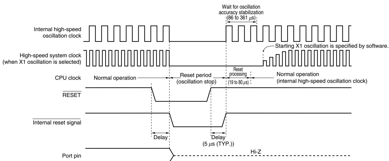
Figure 24-2. Timing of Reset by RESET Input
