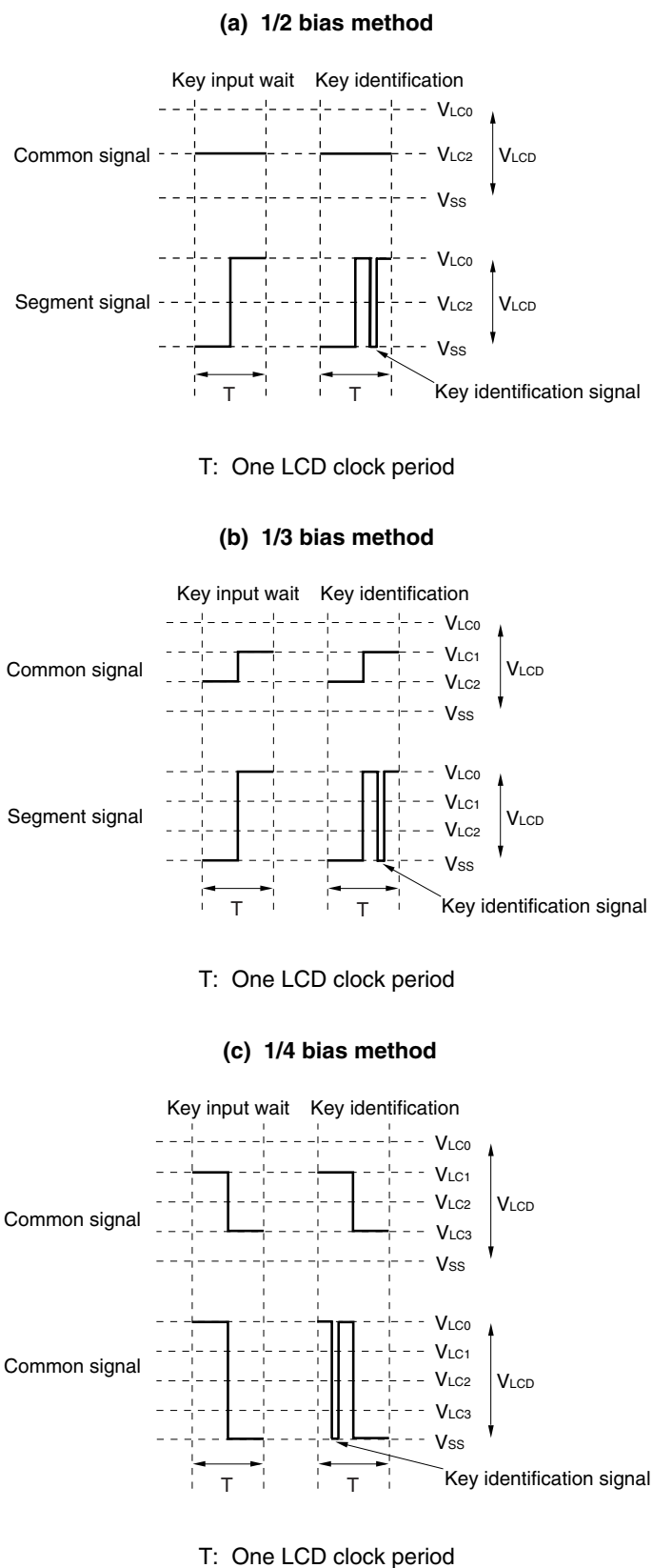
Figure 18-19 Voltages and Phases of Common and Segment Signals
