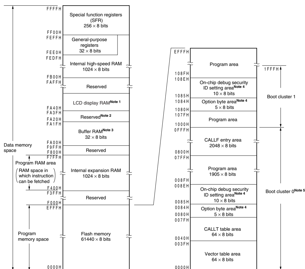
Figure 3-6. Memory Map ( \mu PD78F04x5)
