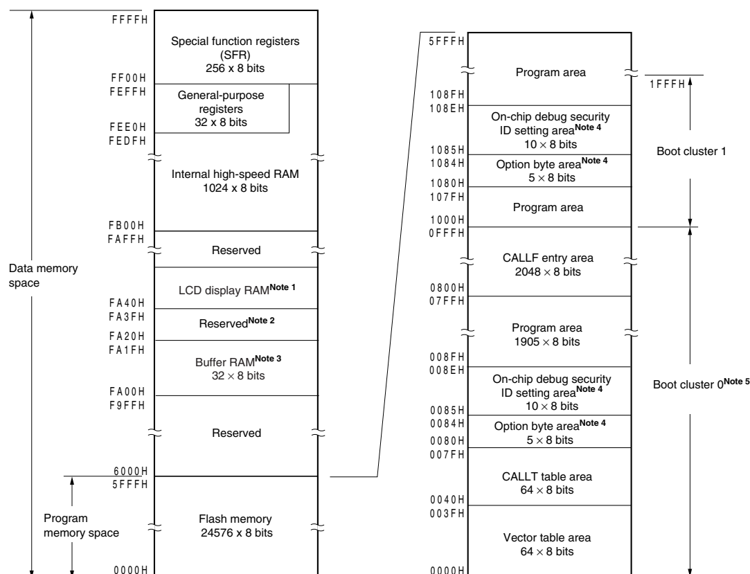
Figure 3-3. Memory Map ( \mu PD78F04x2)
