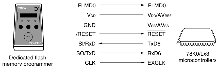
Figure 28-5. Communication with Dedicated Flash memory programmer (UART6)
