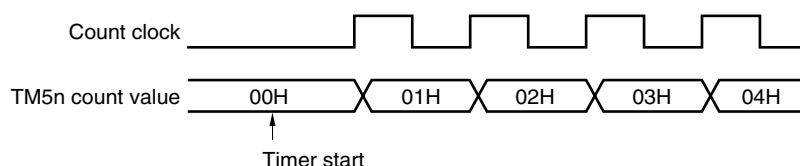
Figure 7-20. 8-Bit Timer Counter 5n (TM5n) Timing
