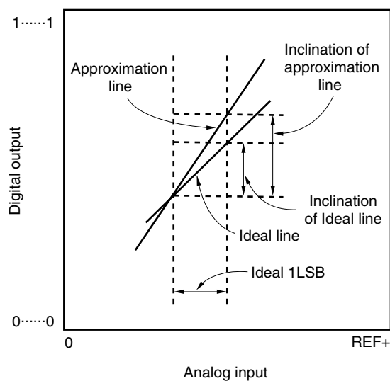
Figure 13-18. Gain Error
