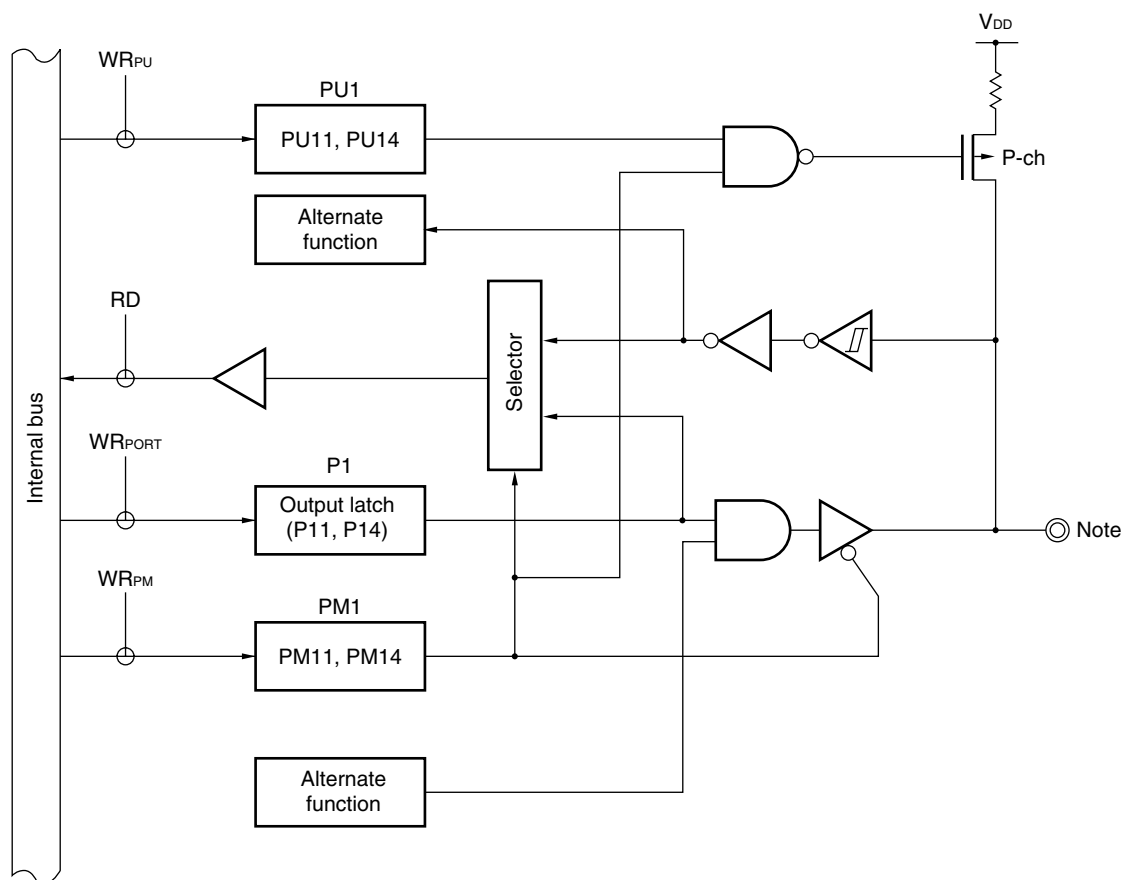
Figure 4-2. Block Diagram of P11 and P14
