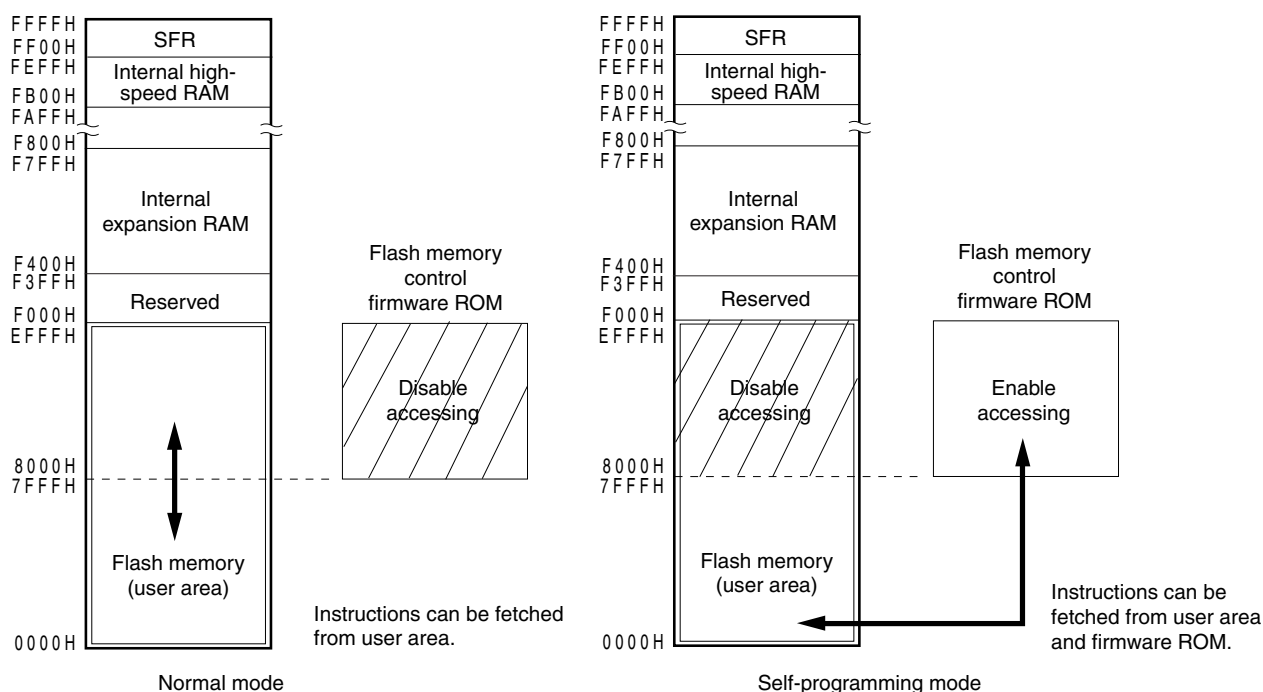
Figure 28-13. Operation Mode and Memory Map for Self-Programming ( \mu PD78F0475)
