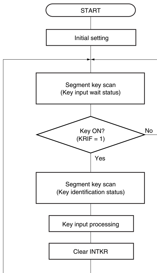
Figure 18-37. Operation Flow of Segment Key Scan
