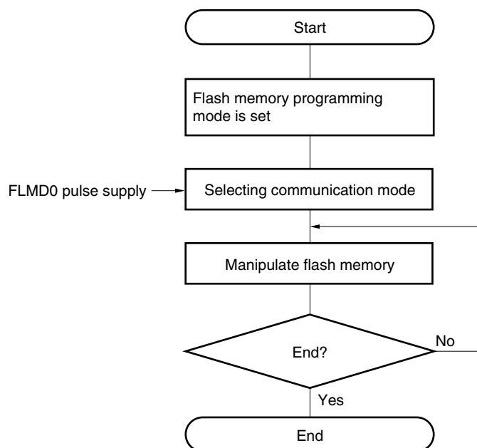
Figure 28-10. Flash Memory Manipulation Procedure
