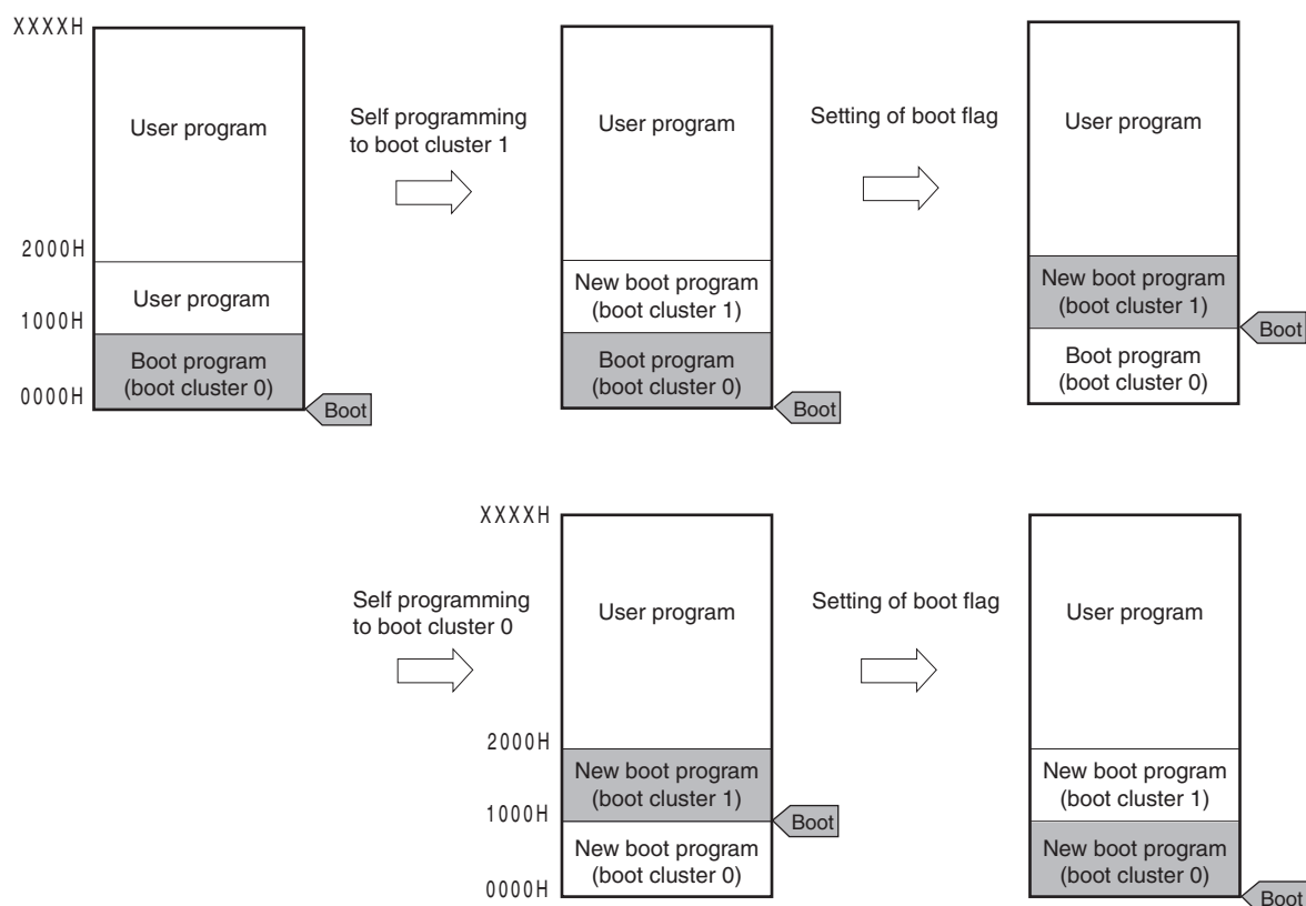
Figure 28-15. Boot Swap Function
