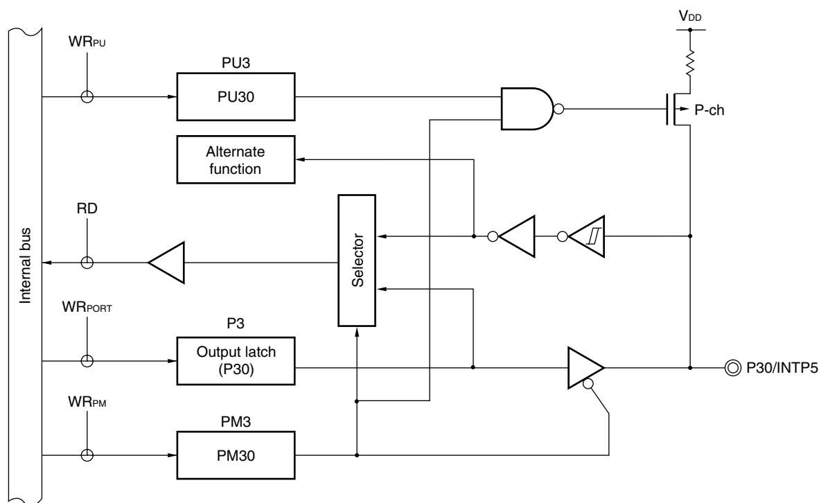
Figure 4-8. Block Diagram of P30
