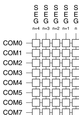
Figure 18-33. Eight-Time-Slice LCD Display Pattern and Electrode Connections
