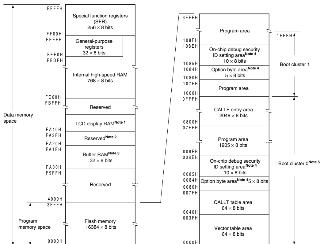
Figure 3-2. Memory Map ( \mu PD78F04x1)
