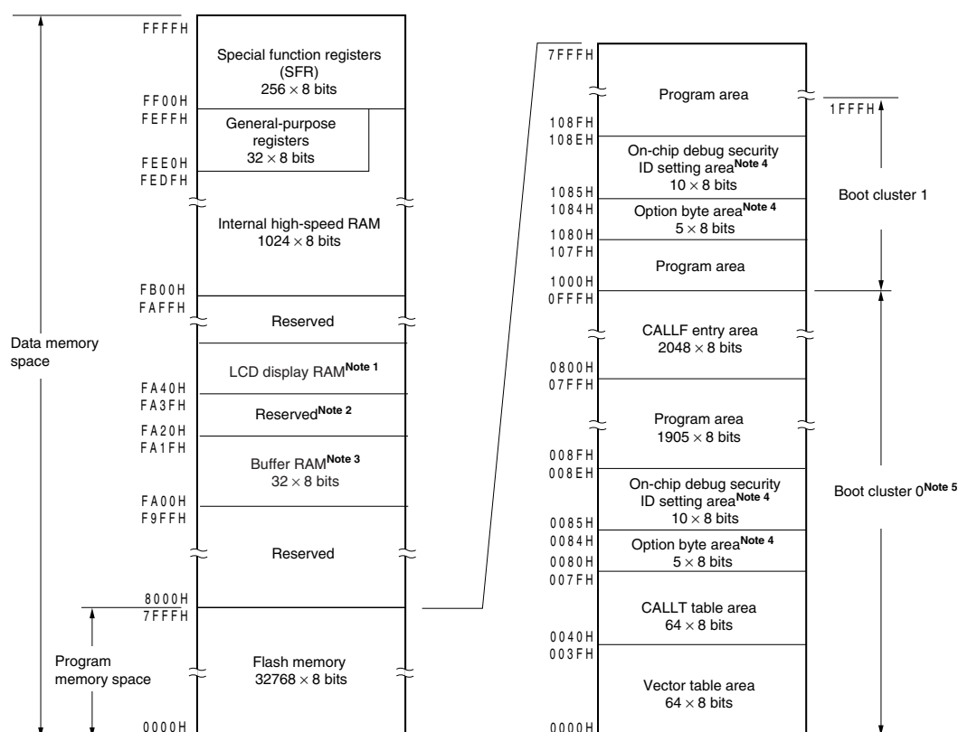
Figure 3-4. Memory Map ( \mu PD78F04x3)
