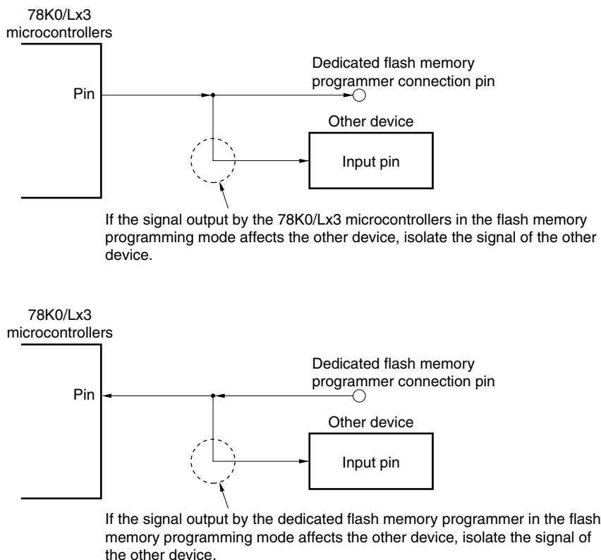
Figure 28-8. Malfunction of Other Device
