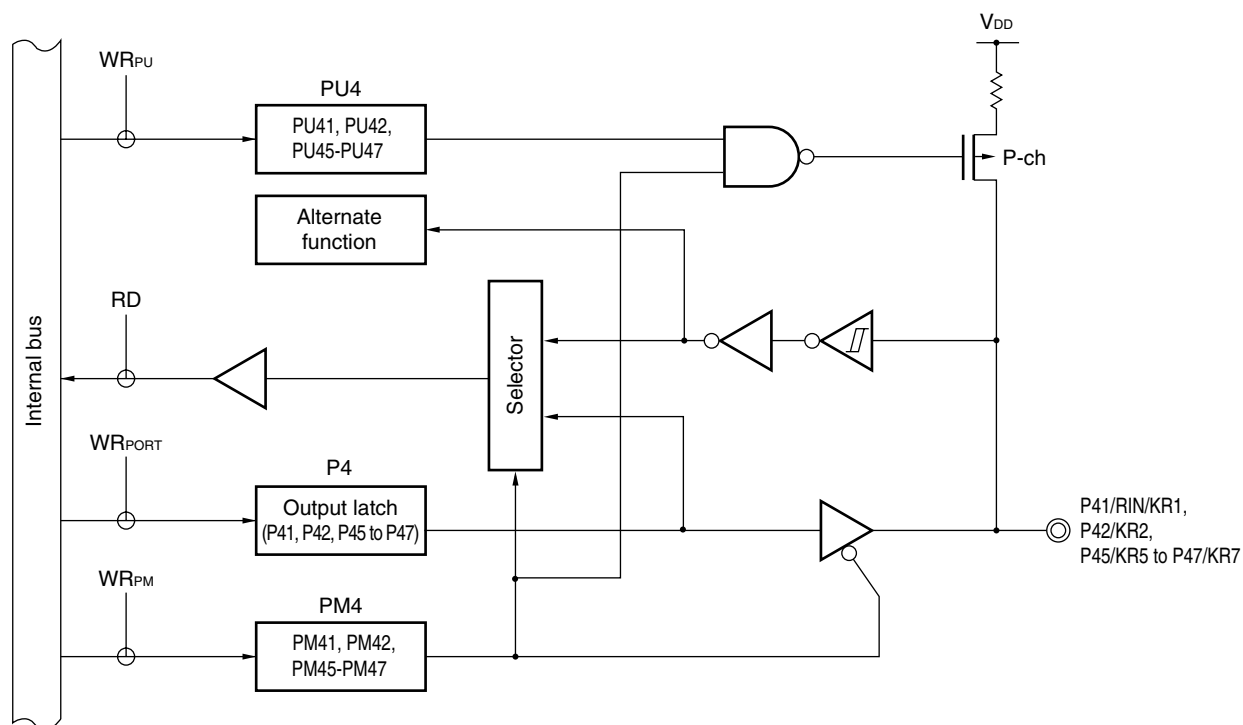
Figure 4-12. Block Diagram of P41, P42, P45 to P47
