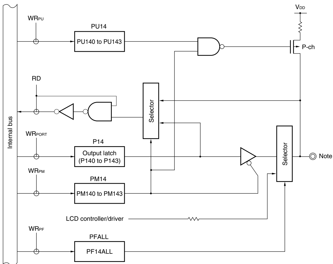
Figure 4-24. Block Diagram of P140 to P143
