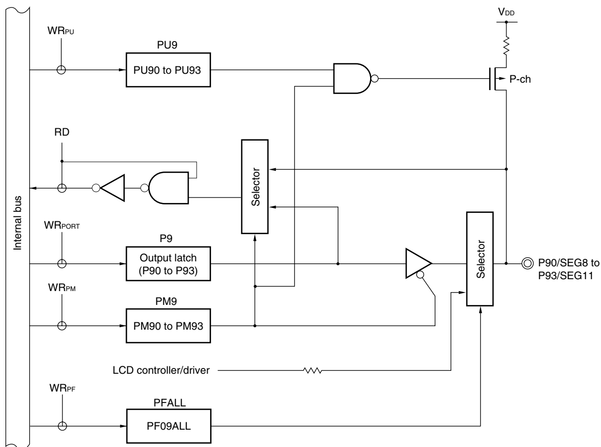
Figure 4-15. Block Diagram of P90 to P93
