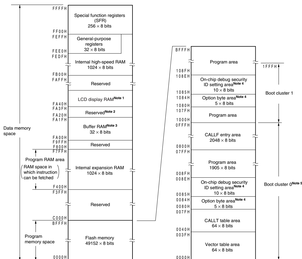
Figure 3-5. Memory Map ( \mu PD78F04x4)
