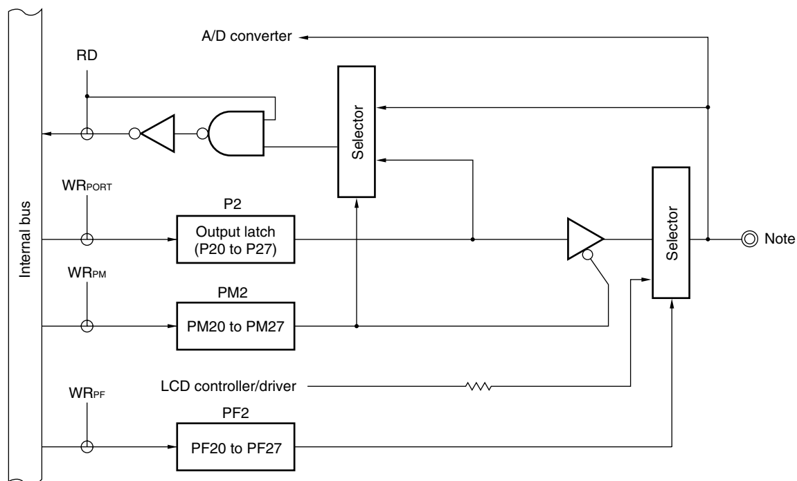
Figure 4-7. Block Diagram of P20 to P27
