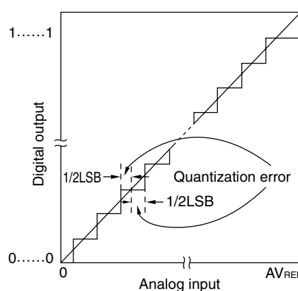
Figure 12-15. Quantization Error
