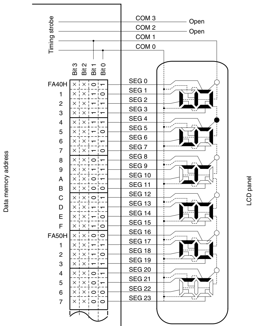
Figure 18-24. Example of Connecting Two-Time-Slice LCD Panel
