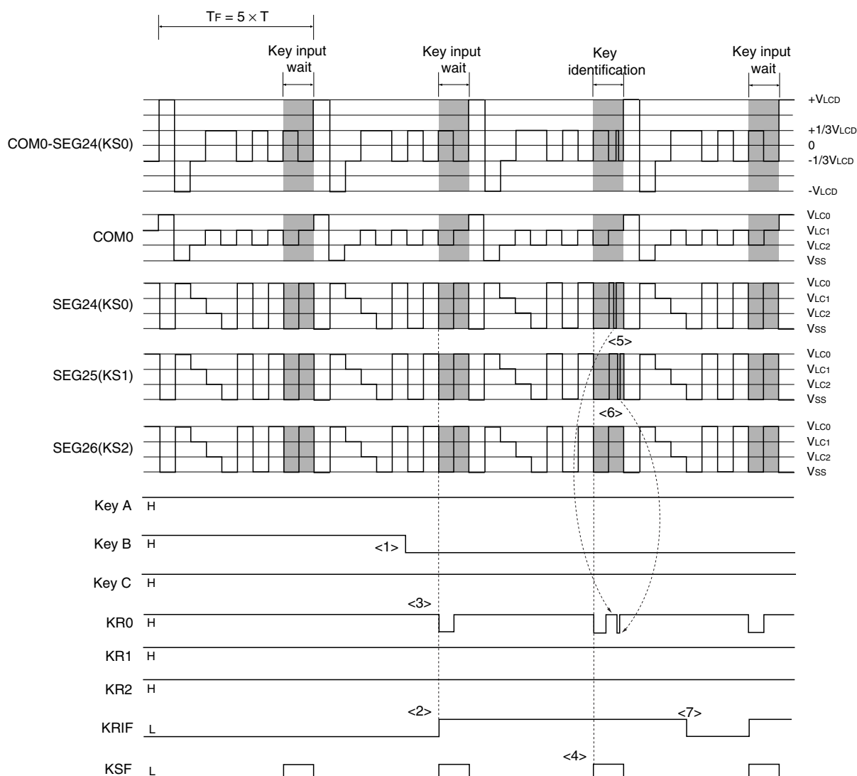
Figure 18-39. Example of Segment Key Scan Operation Timing (Four-Time-Slice (1/3 Bias Method))
