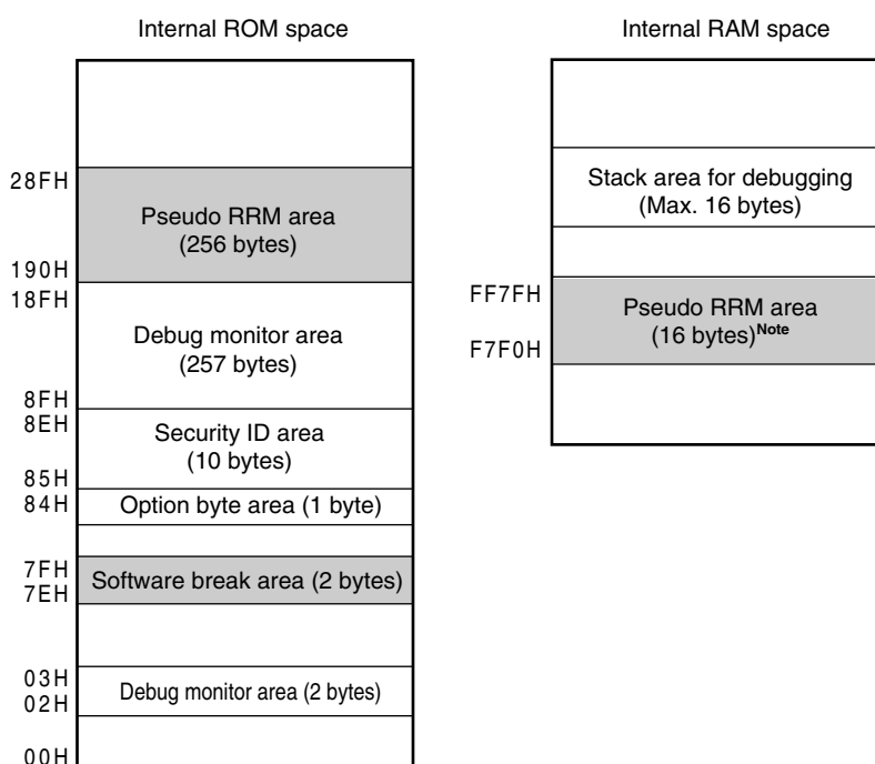
Figure 29-3. Reserved Area Used by QB-MINI2
