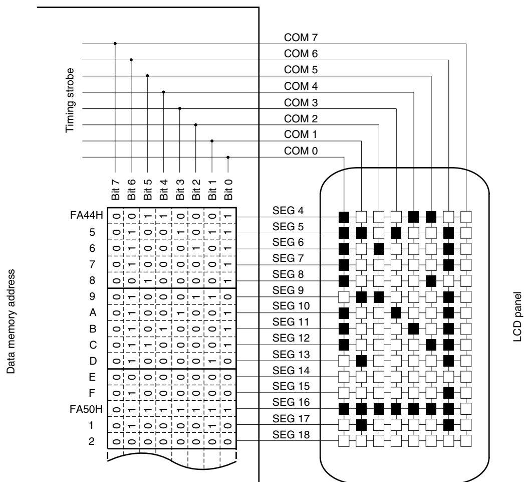
Figure 18-34. Example of Connecting Eight-Time-Slice LCD Panel
