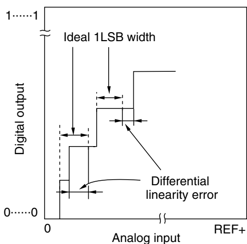
Figure 13-20. Differential Linearity Error
