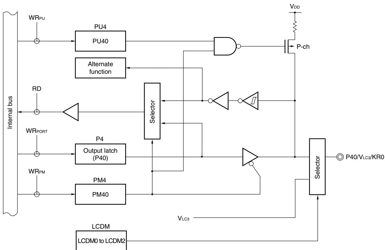
Figure 4-11. Block Diagram of P40
