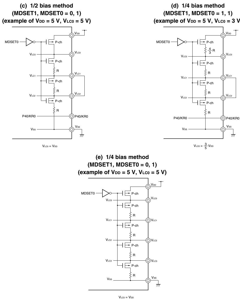
Figure 18-42. Examples of LCD Drive Power Connections (Internal Resistance Division Method) (2/2)
