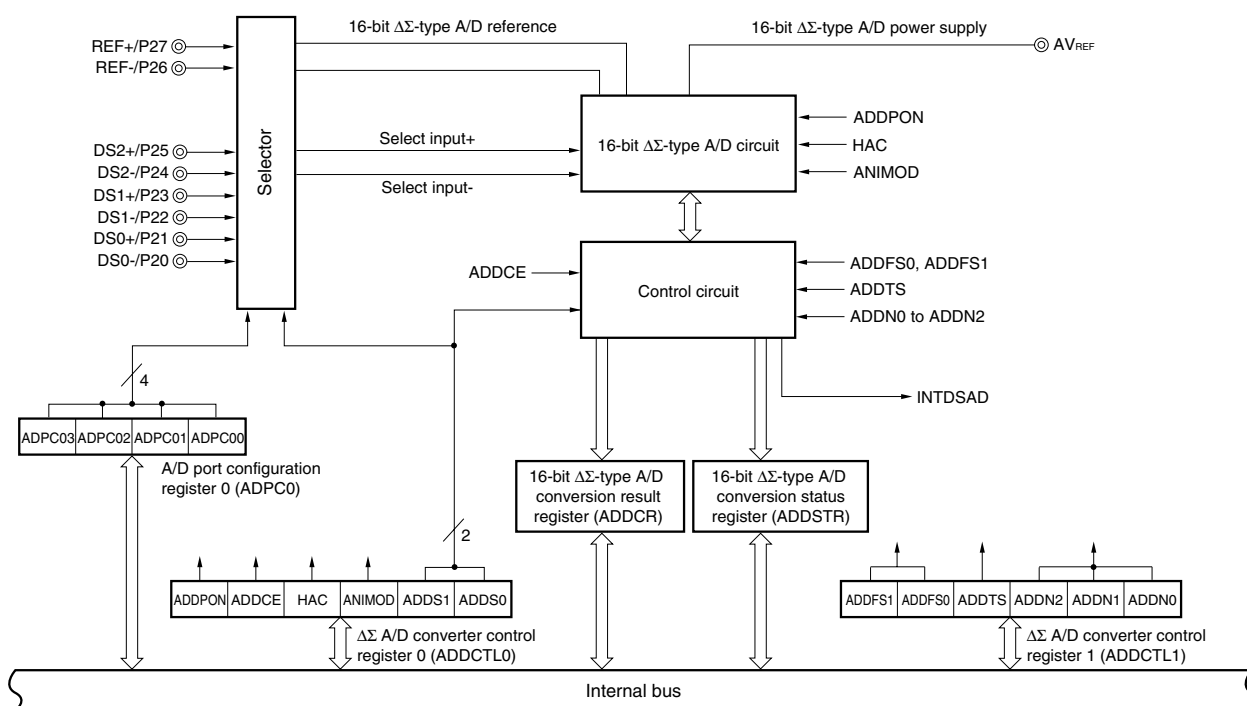
Figure 13-1. Block Diagram of 16-Bit \Delta\Sigma -Type A/D Converter
