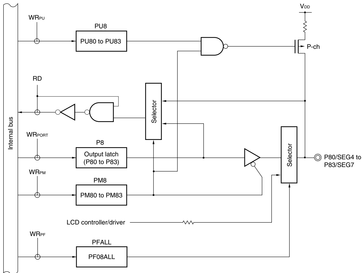
Figure 4-14. Block Diagram of P80 to P83
