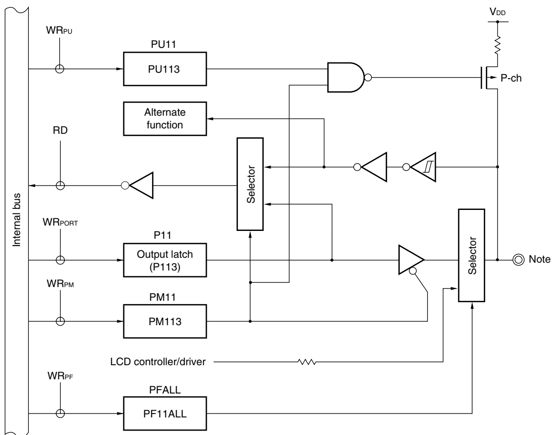
Figure 4-19. Block Diagram of P113
