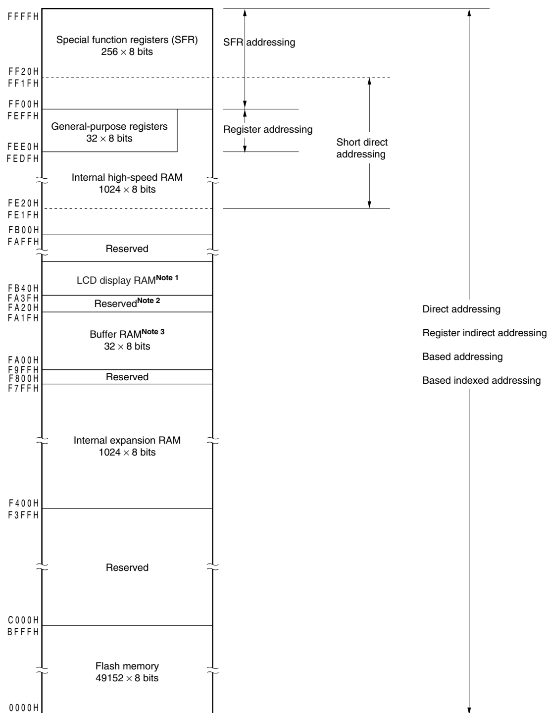
Figure 3-11. Correspondence Between Data Memory and Addressing ( \mu PD78F04x4)
