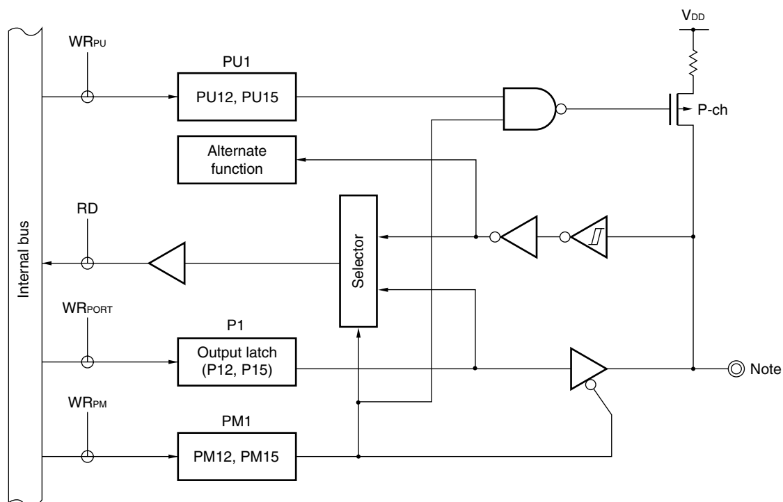
Figure 4-3. Block Diagram of P12 and P15
