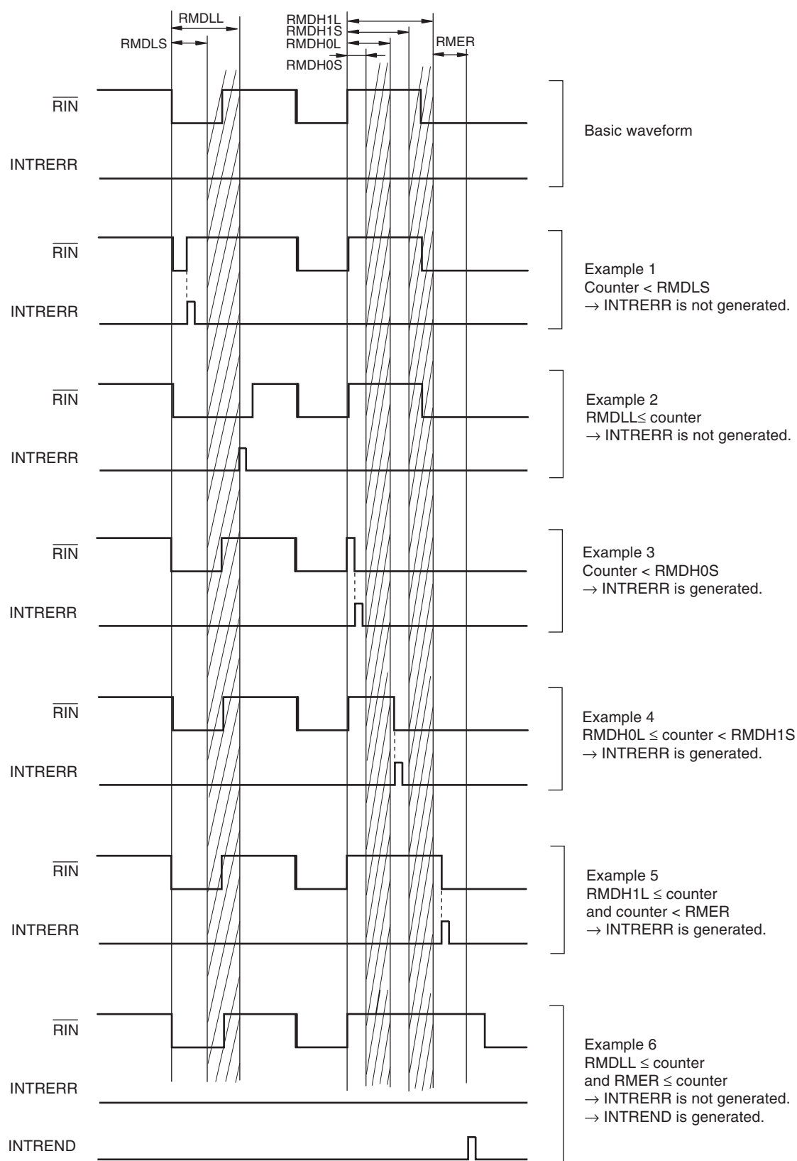
Figure 20-15. Generation Timing of INTRERR Signal (Type C reception mode)
