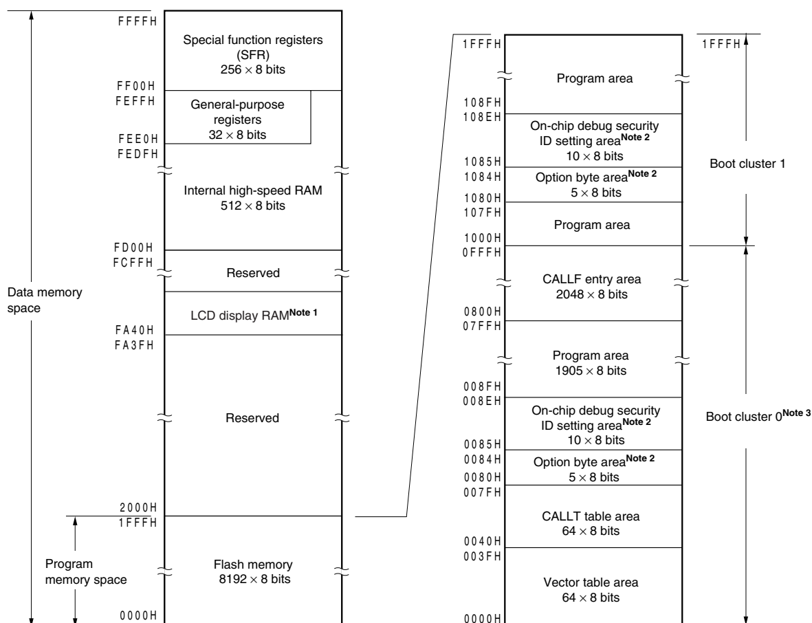
Figure 3-1. Memory Map ( \mu PD78F04x0)
