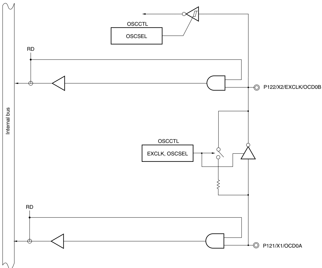
Figure 4-21. Block Diagram of P121 and P122
