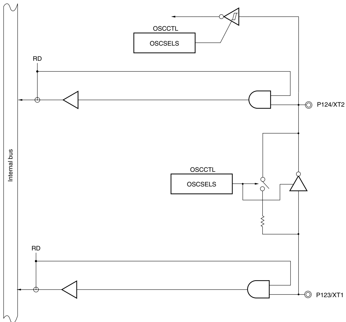
Figure 4-22. Block Diagram of P123 and P124
