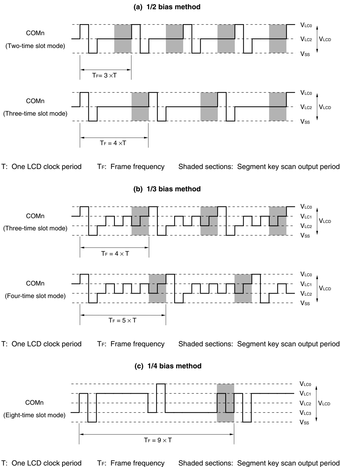
Figure 18-18 Common Signal Waveforms
