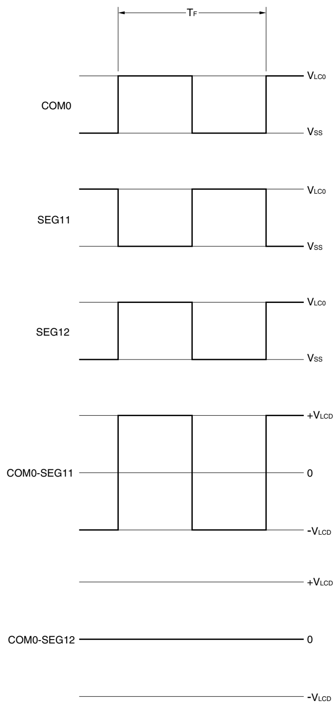
Figure 18-22. Static LCD Drive Waveform Examples
