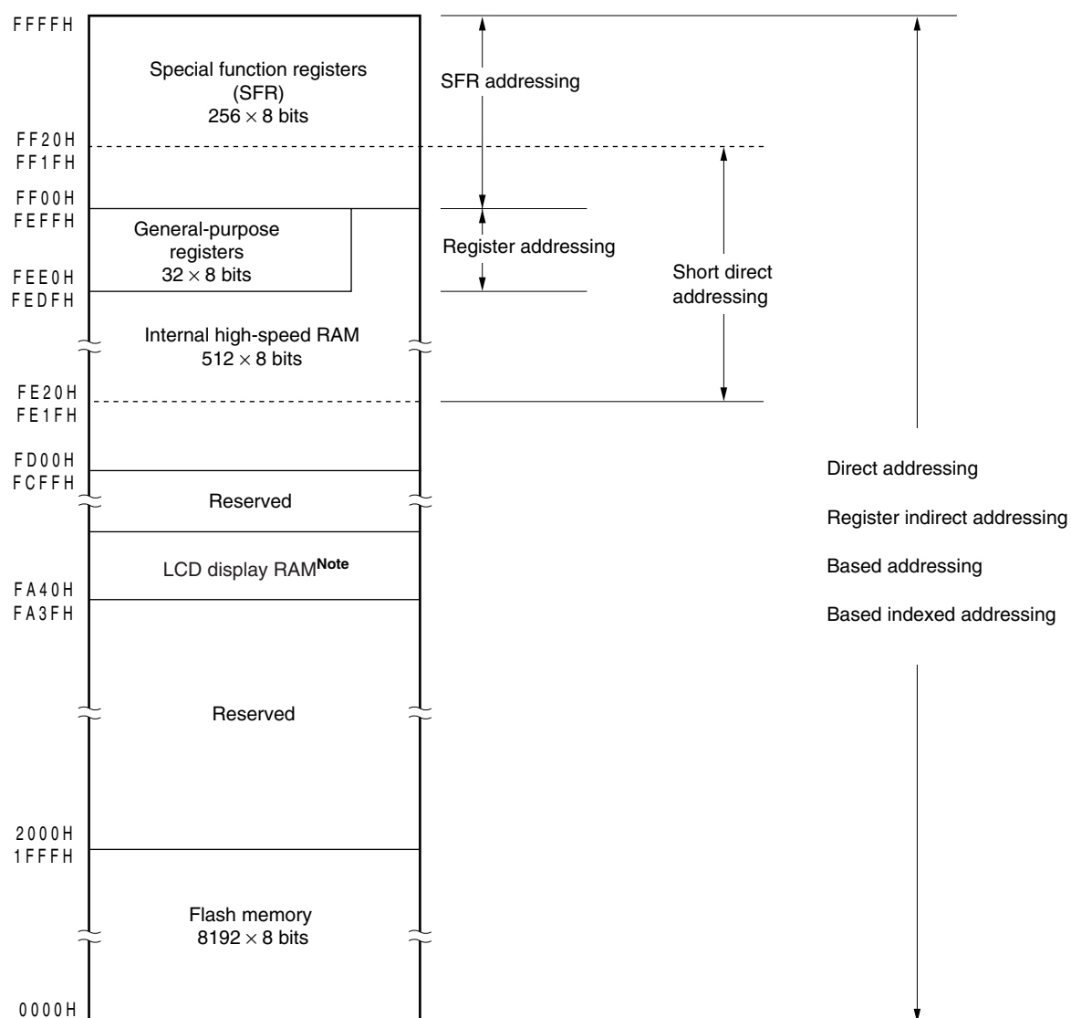
Figure 3-7. Correspondence Between Data Memory and Addressing ( \mu PD78F04x0)
