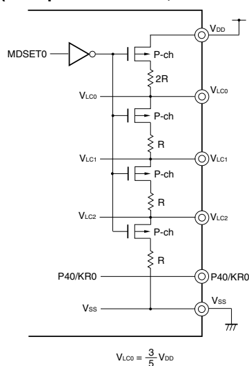
(b) 1/3 bias method and static display mode (MDSET1, MDSET0 = 1, 1) (example of V_{DD} = 5\text{ V} , V_{LC0} = 3\text{ V} )
