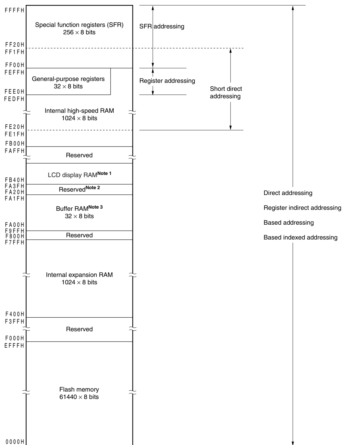
Figure 3-12. Correspondence Between Data Memory and Addressing ( \mu PD78F04x5)
