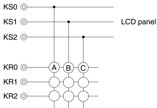
Figure 18-38. Key Connection Example
