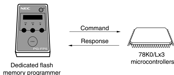
Figure 28-12. Communication Commands
