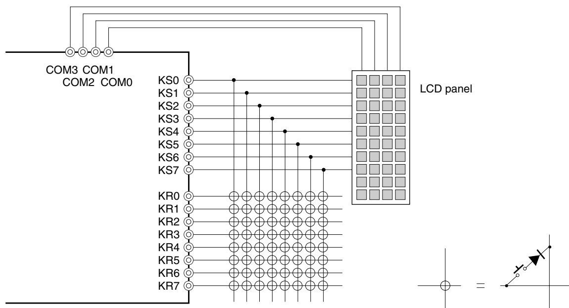
Figure 18-36. Circuit configuration example
