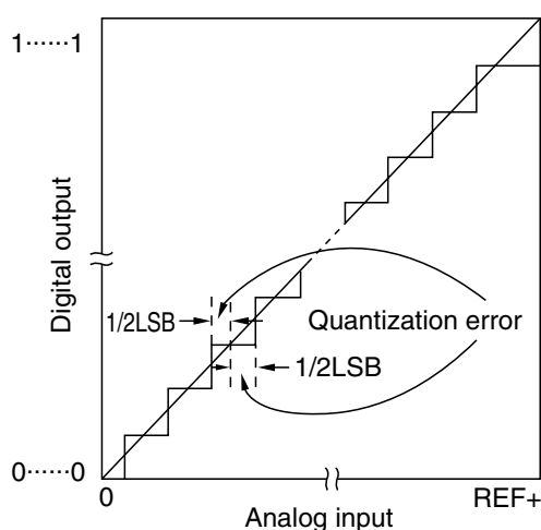
Figure 13-15. Quantization Error
