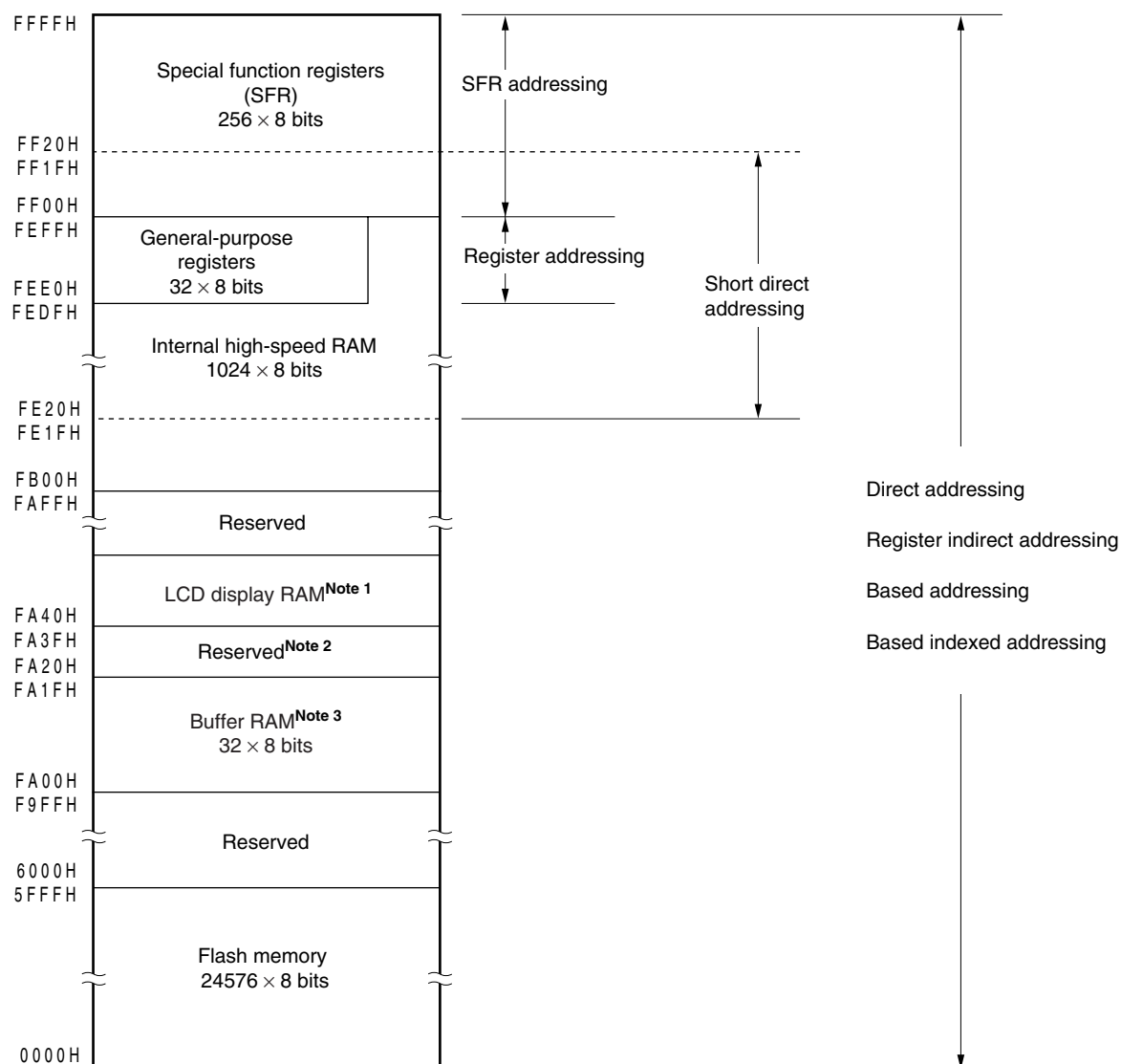
Figure 3-9. Correspondence Between Data Memory and Addressing ( \mu PD78F04x2)
