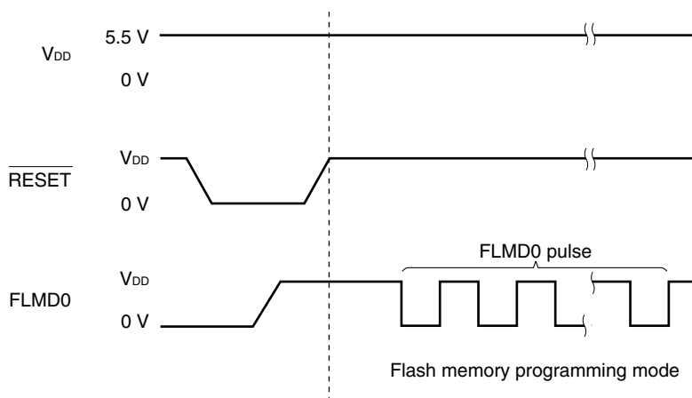
Figure 28-11. Flash Memory Programming Mode
