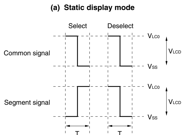
Figure 18-17 Voltages and Phases of Common and Segment Signals
