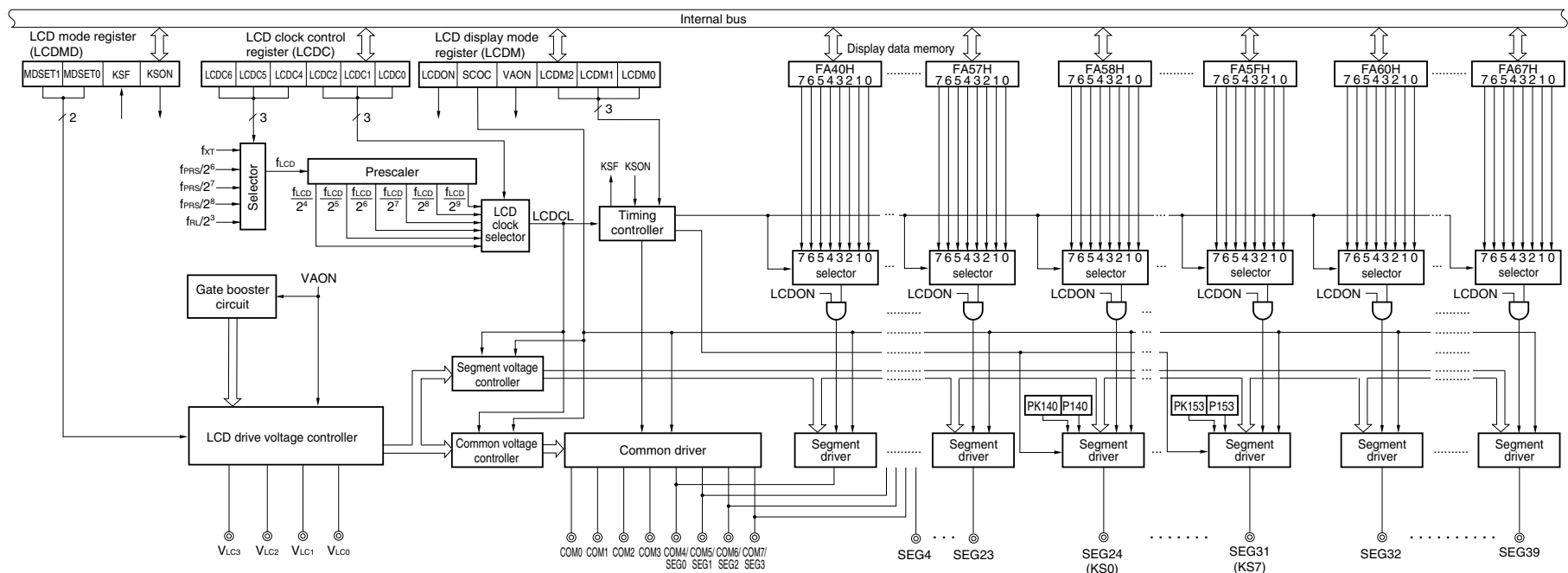
Figure 18-1. Block Diagram of LCD Controller/Driver
