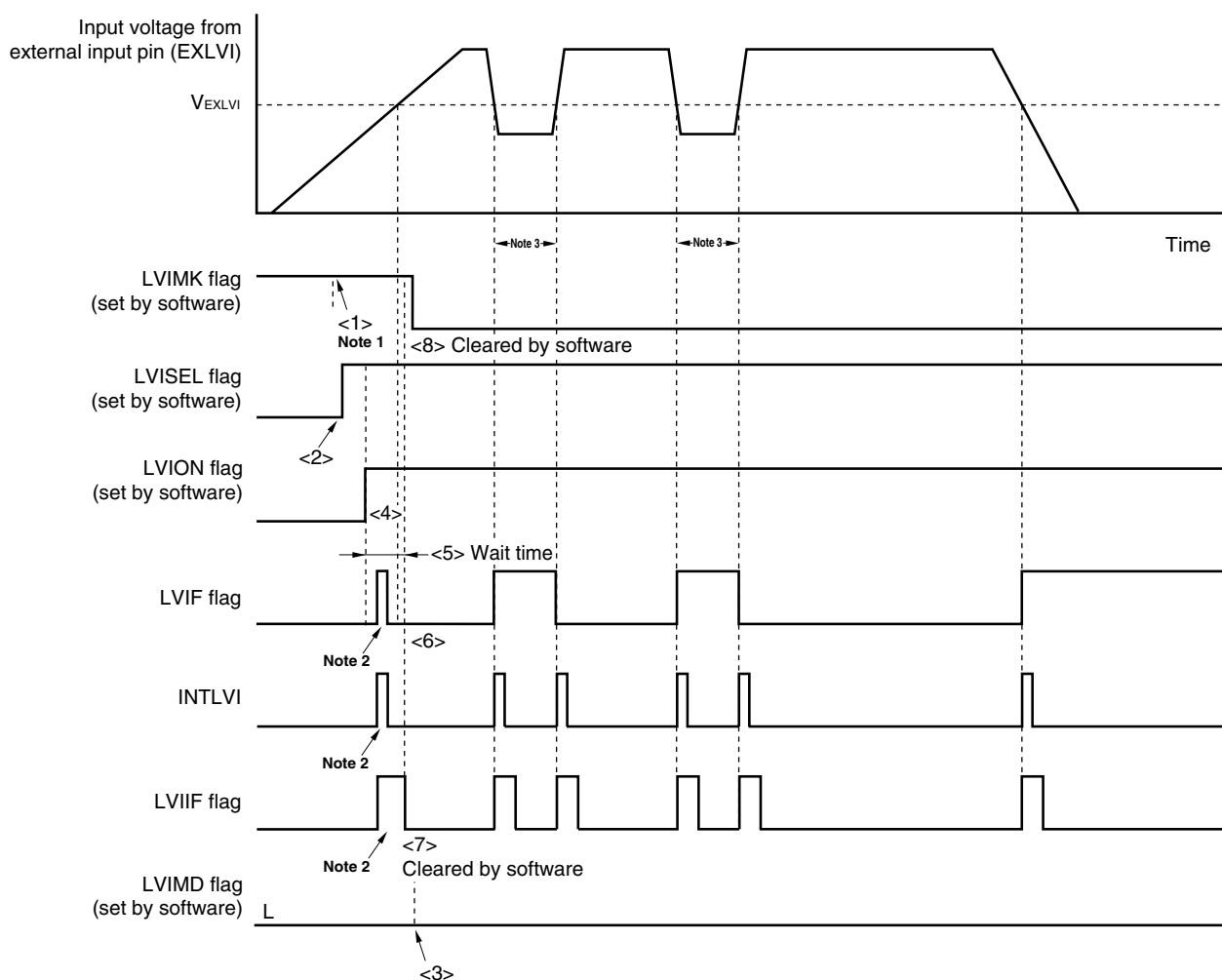
Figure 26-8. Timing of Low-Voltage Detector Interrupt Signal Generation (Detects Level of Input Voltage from External Input Pin (EXLVI))
