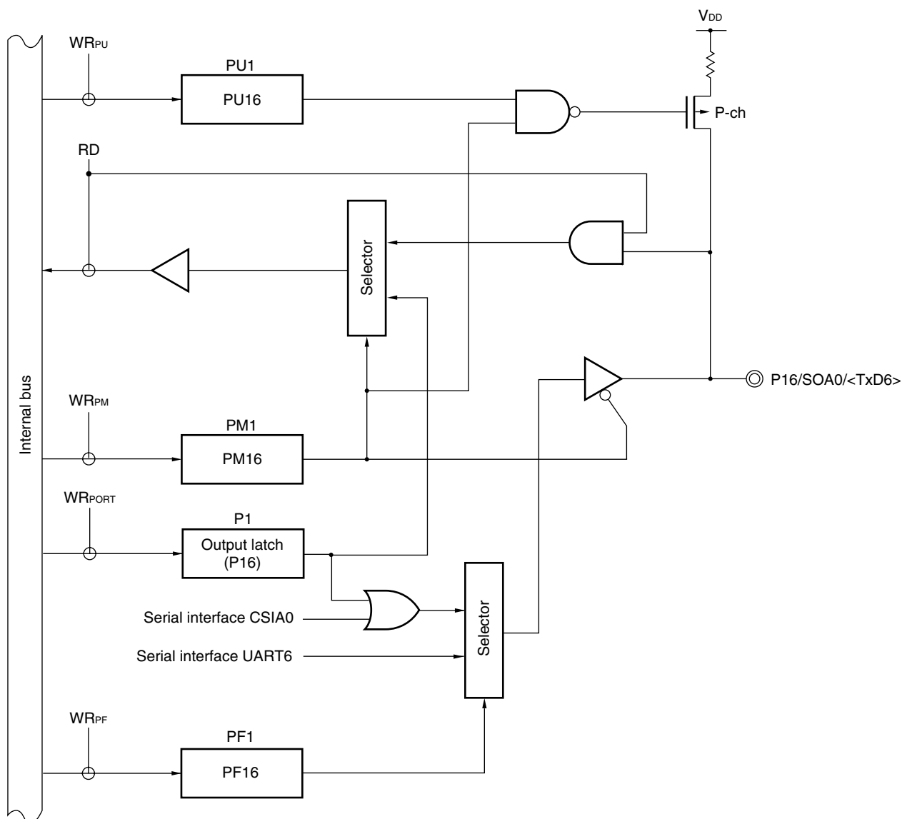
Figure 4-5. Block Diagram of P16
