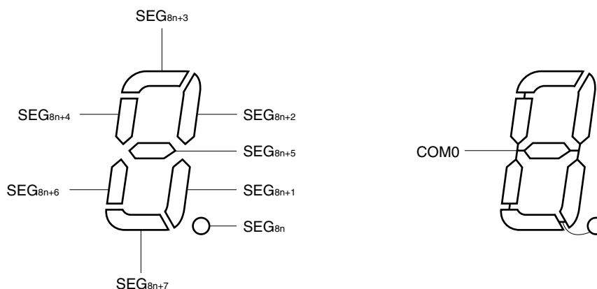
Figure 18-20 Static LCD Display Pattern and Electrode Connections
