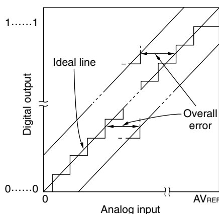
Figure 12-14. Overall Error
