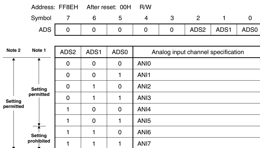
Figure 12-8. Format of Analog Input Channel Specification Register (ADS)
