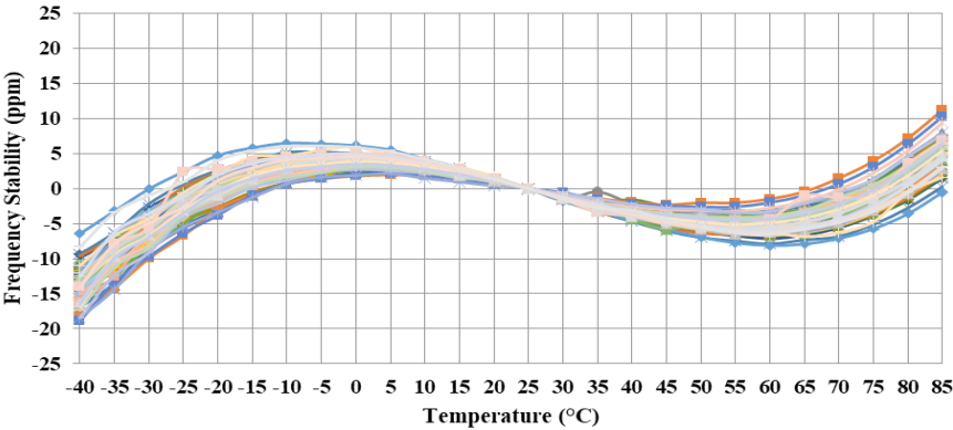
Frequency Stability vs. Temperature AX7PAF1-122.8800 (50 units)
