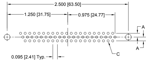
DD78 FEMALE
