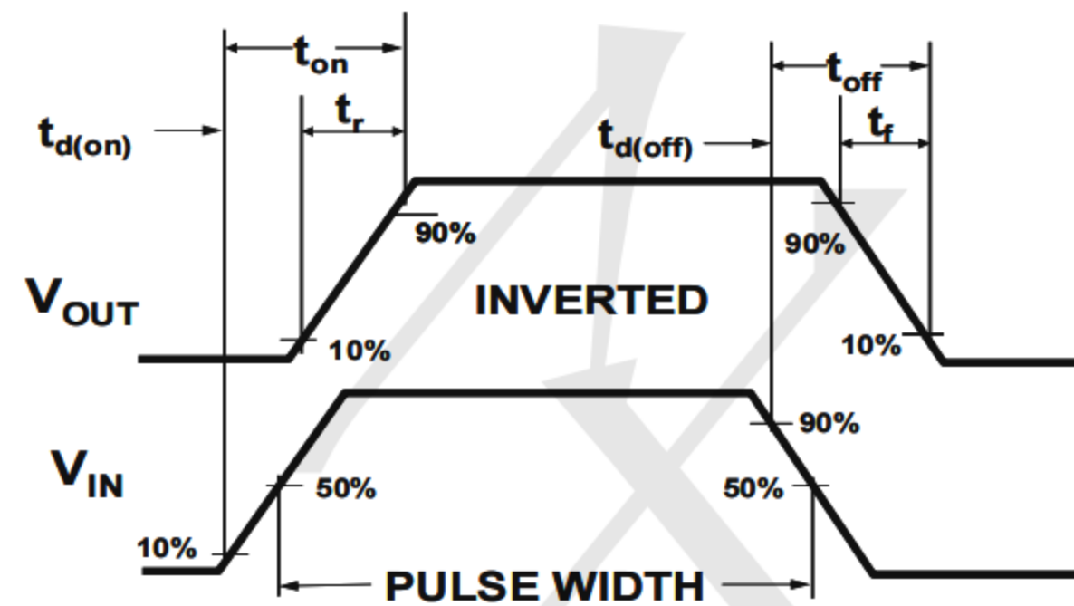
Figure 2:Switching Waveforms
