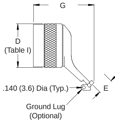
45° ROTATABLE COUPLING
