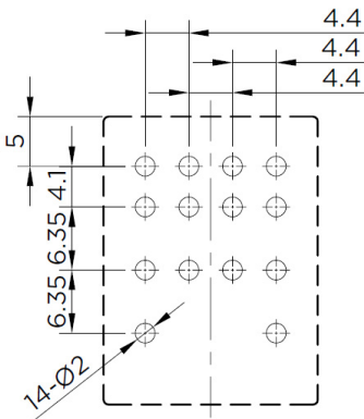
4P PCB socket footprint
