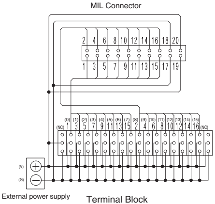
XW2R-P16GD-C3-COM
