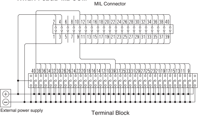
XW2R-P32GD-M2-COM
