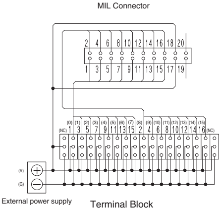
XW2R-P16GD-C1-COM
