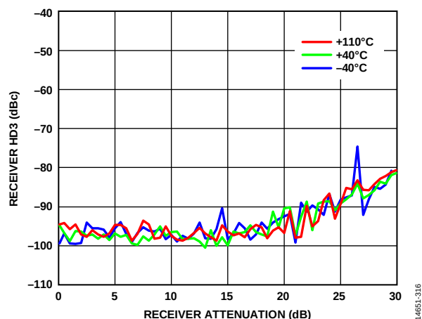
Figure 16. Receiver HD3 vs. Receiver Attenuation, 800 MHz LO, CW Signal 3 MHz Offset, -20 dBm at 0 dB Attenuation, Input Power Increasing Decibel for Decibel with Attenuation, 20 MHz RF Bandwidth, 30.72 MSPS Sample Rate
