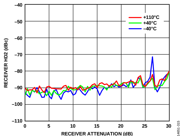
Figure 15. Receiver HD2 vs. Receiver Attenuation, 800 MHz LO, CW Signal 3 MHz Offset, -20 dBm at 0 dB Attenuation, Input Power Increasing Decibel for Decibel with Attenuation, 20 MHz RF Bandwidth, 30.72 MSPS Sample Rate
