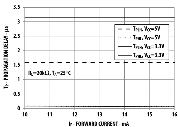
Figure 10. Propagation Delay Time vs Input Current
