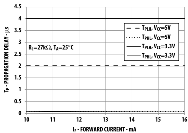
Figure 12. Propagation Delay Time vs Input Current
