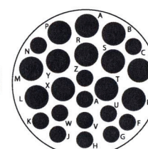
25-24 24-24† 25-24 No. of Contacts 12 #16, 12 #12 Service Ratings I
