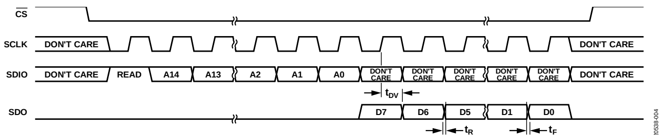
Figure 4. SPI 4-Wire Read Timing Diagram
