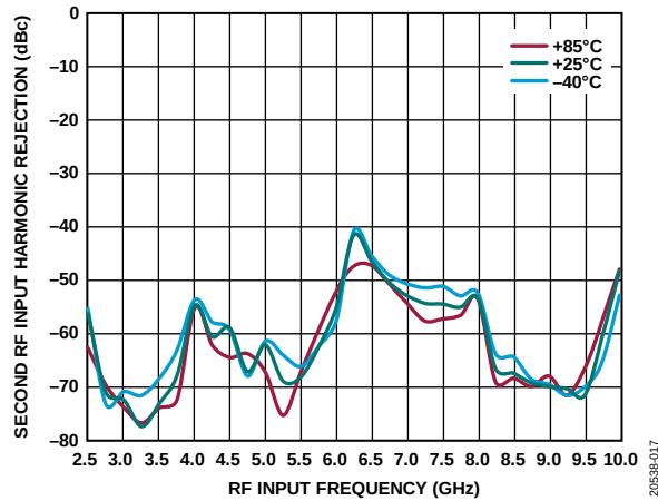
Figure 14. Second RF Input Harmonic Rejection vs. RF Input Frequency and Temperature
