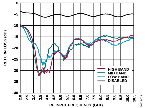
Figure 22. RF Input Return Loss
