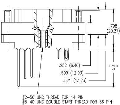
RECEPTACLE WITH LOCKNUT AND POLARIZING SOCKETS
