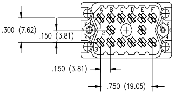
14 PIN PLUG
