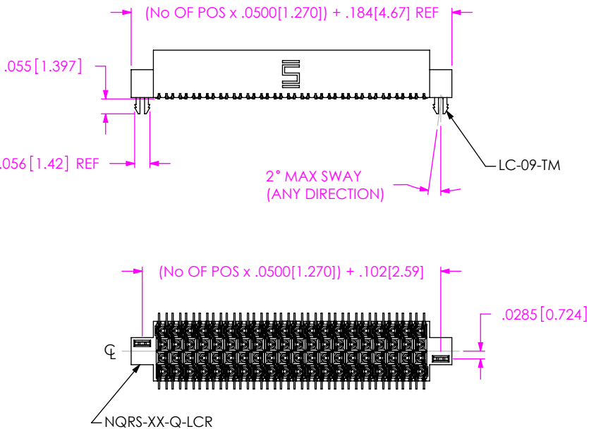
FIG 2 -LCR: LOCKING CLIP REVERSED [DIFFERENT AS SHOWN, OTHERWISE SAME AS FIG 1]
