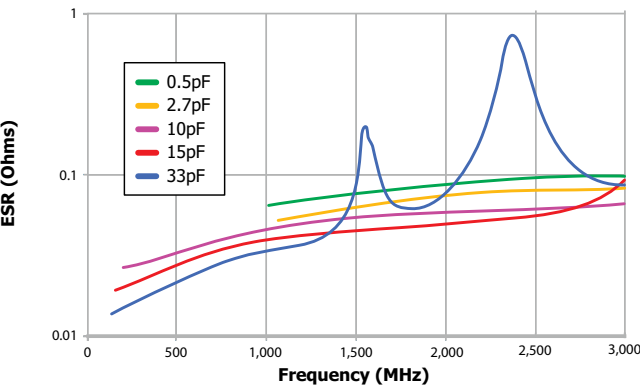
Q Series — ESR vs. Frequency — Case Size 0505
