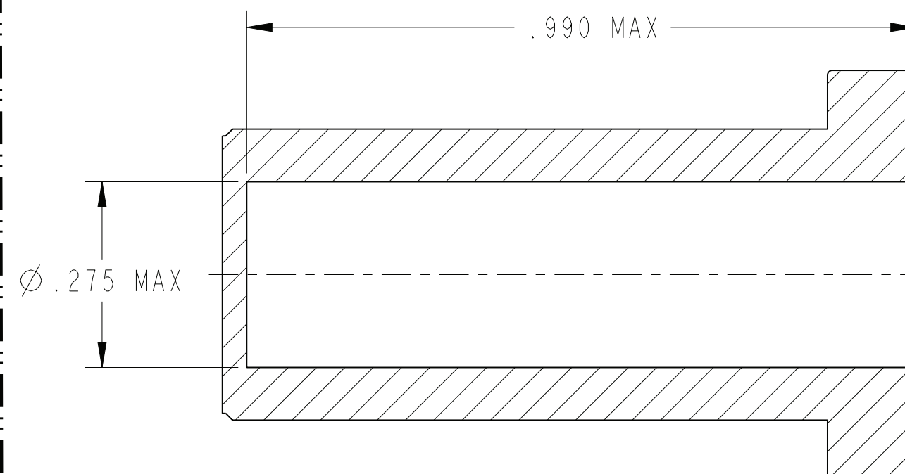
OPTIONAL DESIGN FOR 10-405996-03 (MS27488-0-3)
