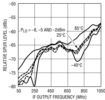
2RF-LO Spur vs IF Output Frequency ( P_{RF} = -12\text{dBm} )
