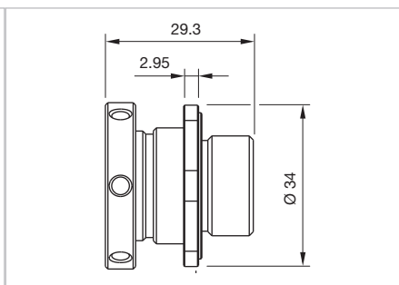
Dimensions [mm] for Part No. 45-50D.2900
