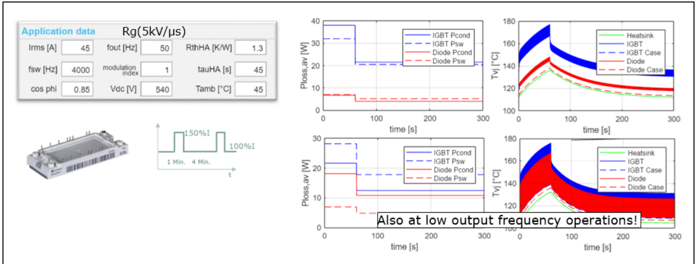
Figure 13. Power losses and Temperature profile under heavy duty load profile
