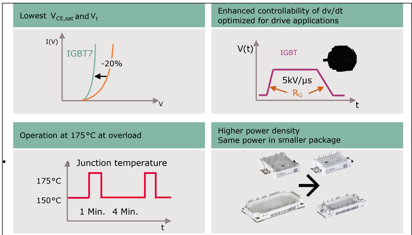
Figure 1. Key technical benefits of TRENCHSTOP™ IGBT7
