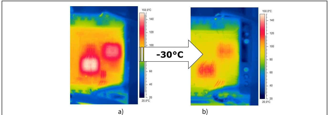
Figure 14. H-bridge inverter test and comparison of junction temperatures for a) IGBT4 and b) IGBT7 at the same output current
