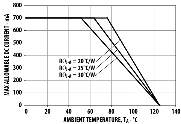
Figure 10. Maximum Forward Current vs. Ambient Temperature. Derated based on T_{JMAX} = 125^\circ\text{C} , R_{\theta JA} = 20^\circ\text{C/W} , 25^\circ\text{C/W} and 30^\circ\text{C/W} .
