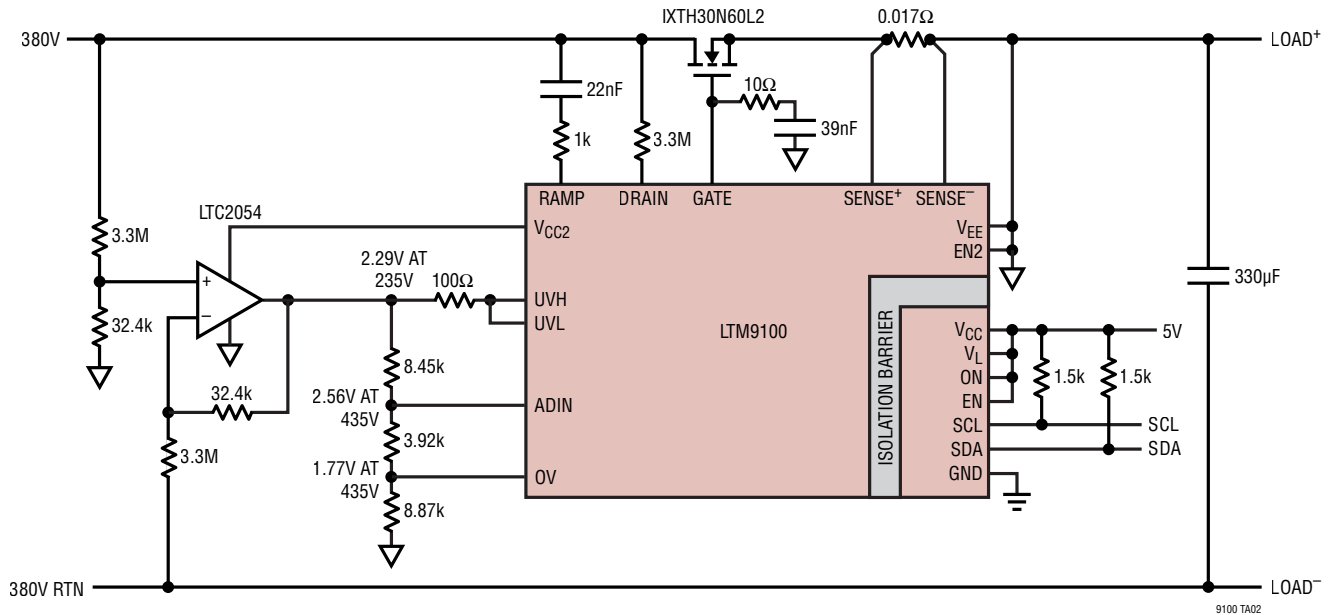
High Side 380V Bus Inrush Current Limiter with Line Voltage Monitor and I 2 C Only Control
