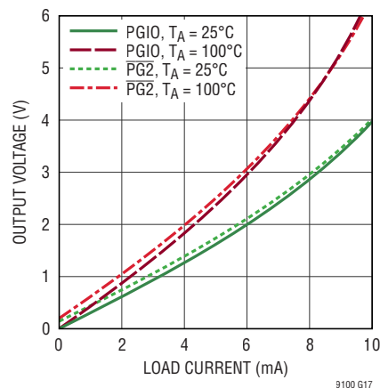
\overline{\text{PG2}} , \overline{\text{PGIO}} Output Low Voltage vs Load Current
