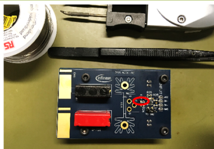
Step 5 MOSFETs placement into the socket
