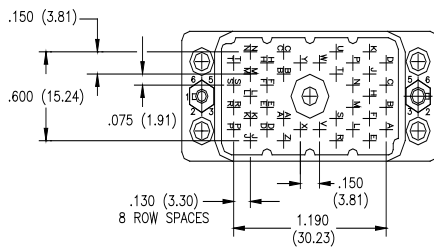
38 PIN PLUG
