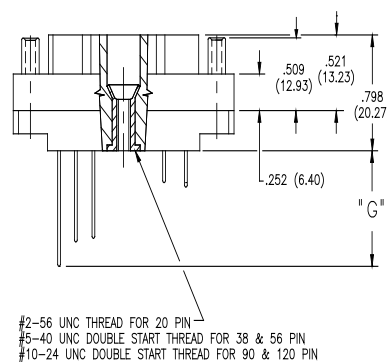
TYPICAL RECEPTACLE WITH LOCKNUT AND POLARIZING SOCKETS
