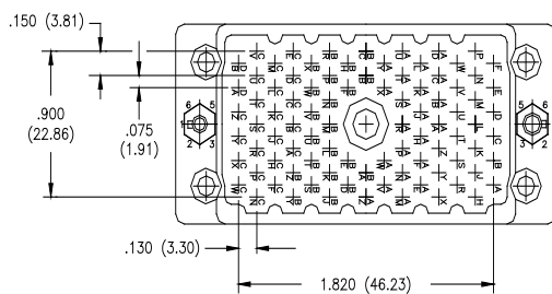
90 PIN PLUG
