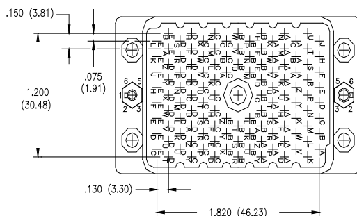
120 PIN PLUG
