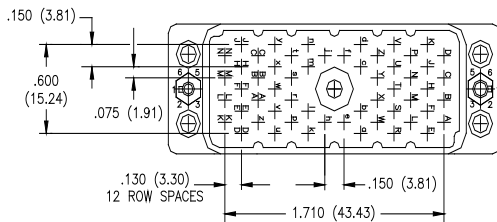
56 PIN PLUG
