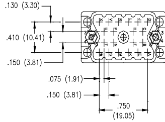
20 PIN PLUG
