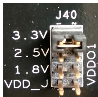
Figure 18. Power Source Selection
