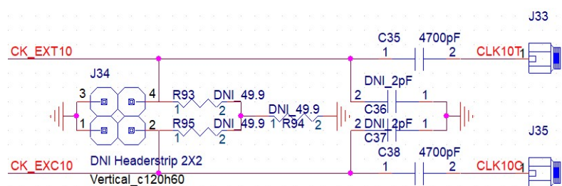
Figure 16. Output Termination with Bias Schematic
