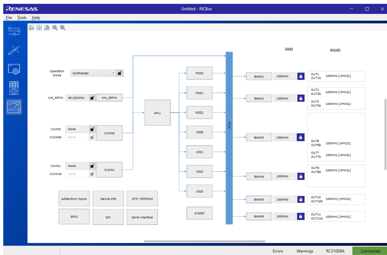
Figure 28. Block Diagram
