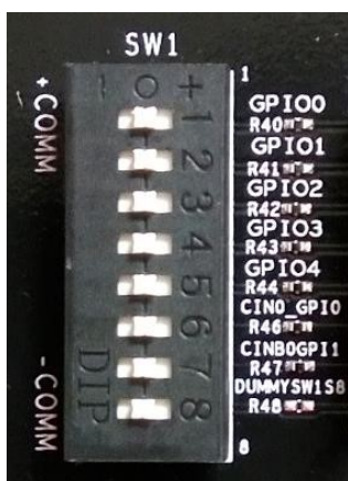
Figure 13. DIP Switch SW1
