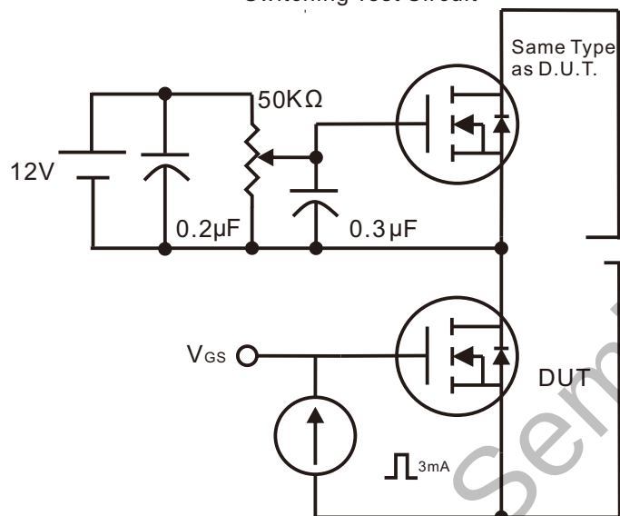
Switching Test Circuit
