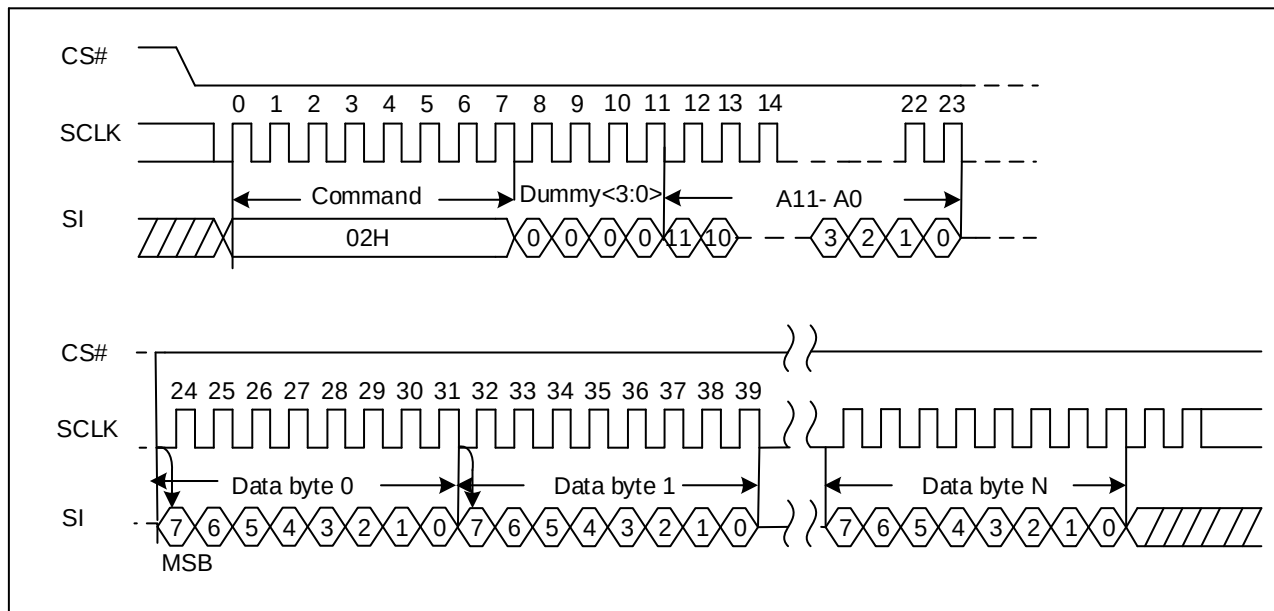
Figure 9-1. Program Load Sequence Diagram
