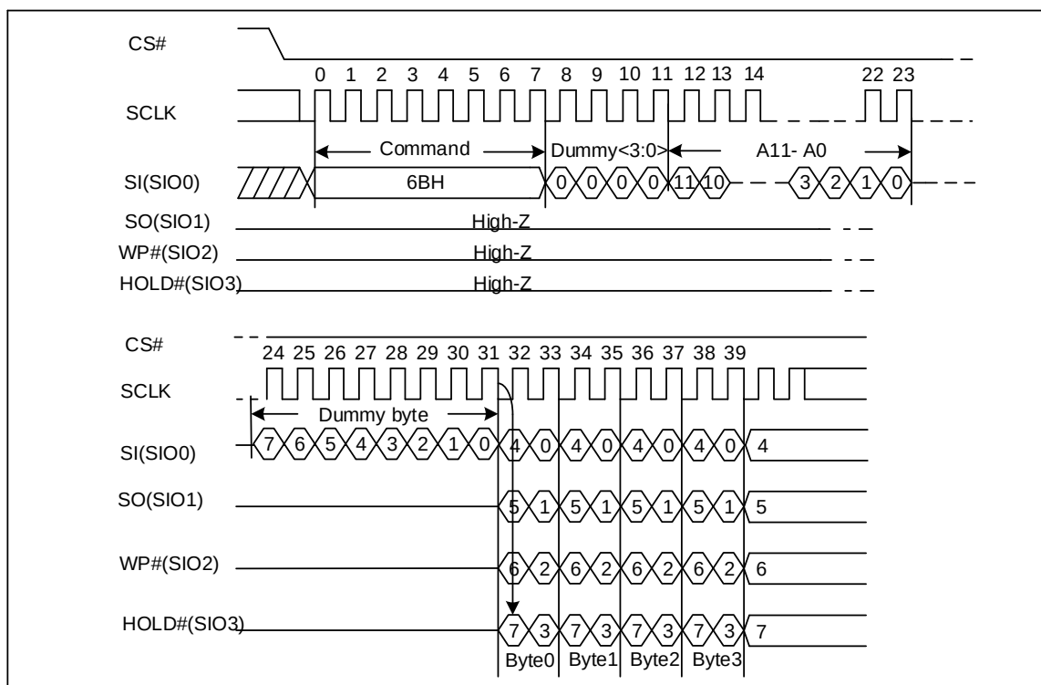
Figure 8-4. Read From Cache x4 Sequence Diagram
