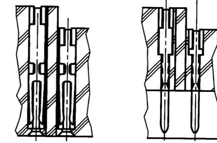
SOCKET PIN SECT. A-A (SCALE 2:1)
