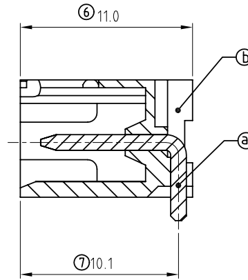
SECTION P-P
