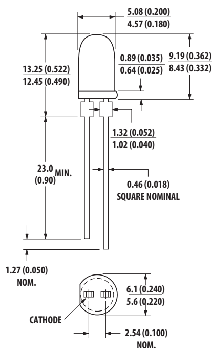
Package Outline B
