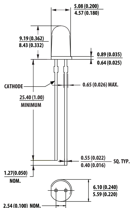
Package Outline A
