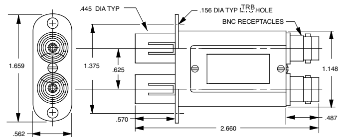
J74T-R Self-Terminating
