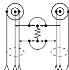
J74T-R Self-Terminating
