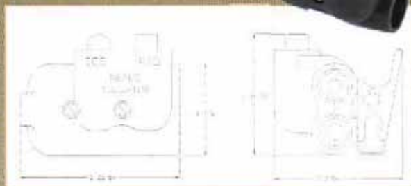
Telephone Jack, Two Switches Bixial Shielded, Six Conductor
