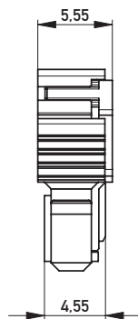
Cover loose mounted
