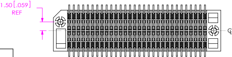
FIG.1 FOR POSITIONS -10, -20, -30 & -35 (SHOWN: MEC8-130-01-XX-DV-XX AS NOTED)
