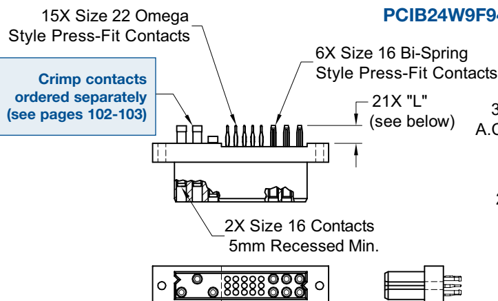
CONNECTOR DIMENSIONS
