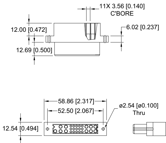
CONNECTOR DIMENSIONS
