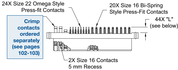
CONNECTOR DIMENSIONS
