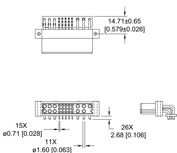
CONNECTOR DIMENSIONS
