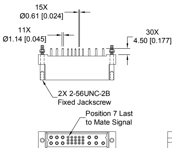
CONNECTOR DIMENSIONS
