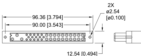
CONNECTOR DIMENSIONS
