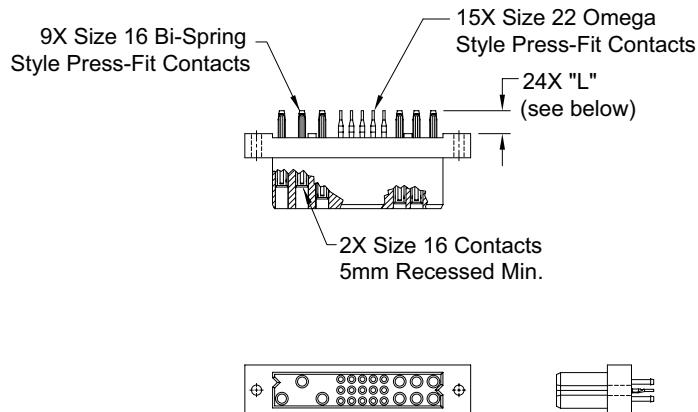
CONNECTOR DIMENSIONS
