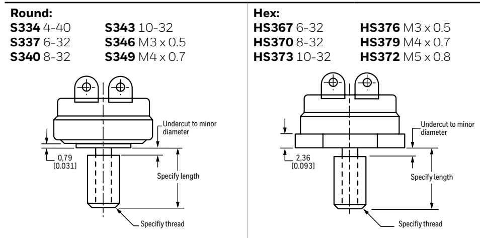
Figure 5: 3001/3004 Series Cap Studs
