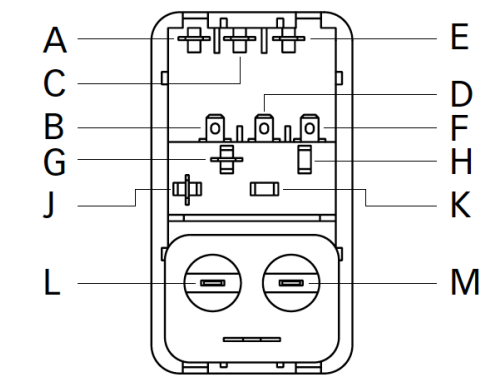
Connection designation
