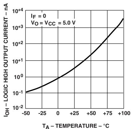
Figure 6. Logic high output current vs. temperature.
