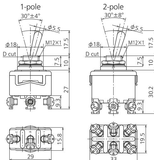
External dimensions
