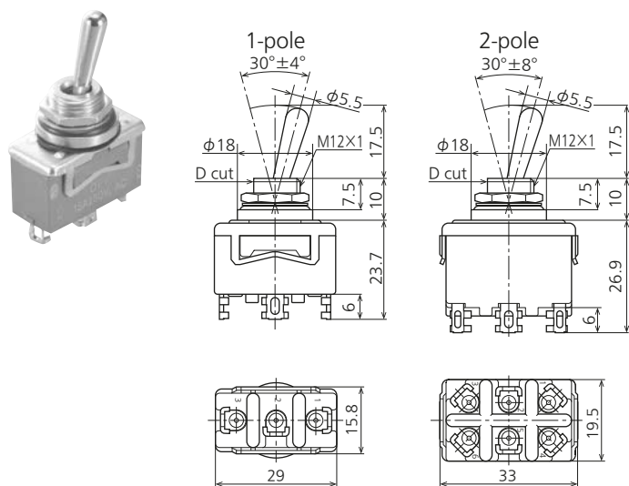
External dimensions
