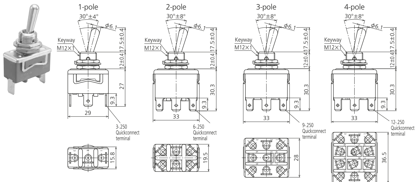
External dimensions
