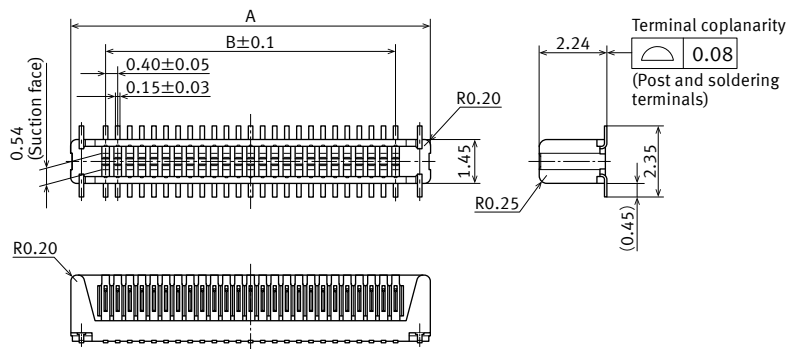
Soldering terminals
