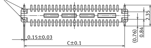
Soldering terminals
