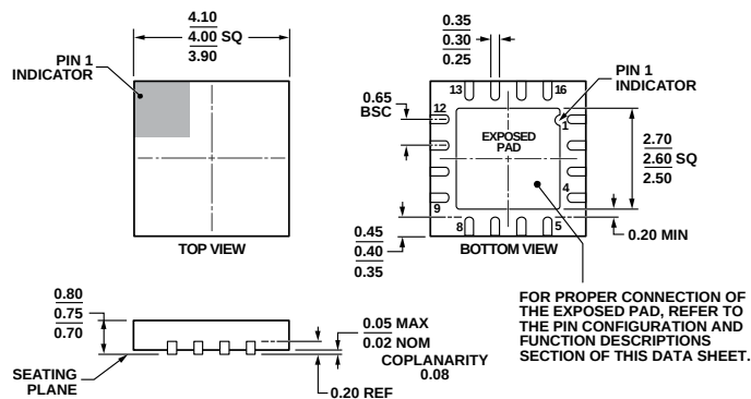
COMPLIANT TO JEDEC STANDARDS MO-220-WGGC. Figure 64. 16-Lead Lead Frame Chip Scale Package [LFCSP_WQ] 4 mm × 4 mm Body, Very Very Thin Quad (CP-16-17) Dimensions shown in millimeters
