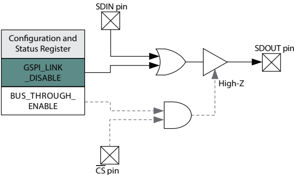
Figure 4-20: GSPI_LINK_DISABLE Operation
