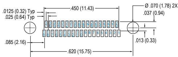
37 Contacts
