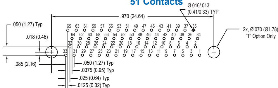
51 Contacts
