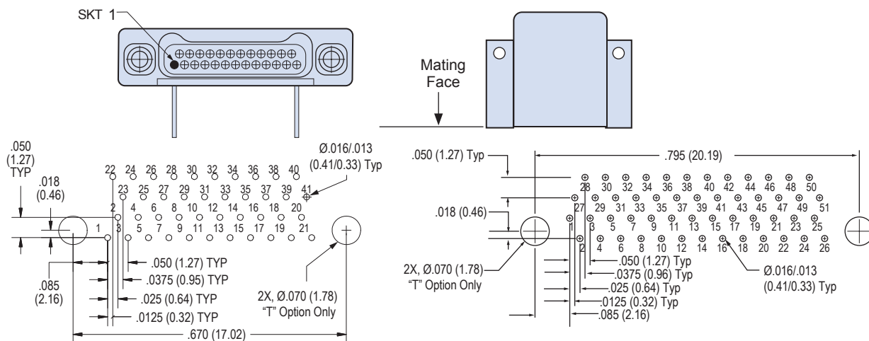
51 Contacts
