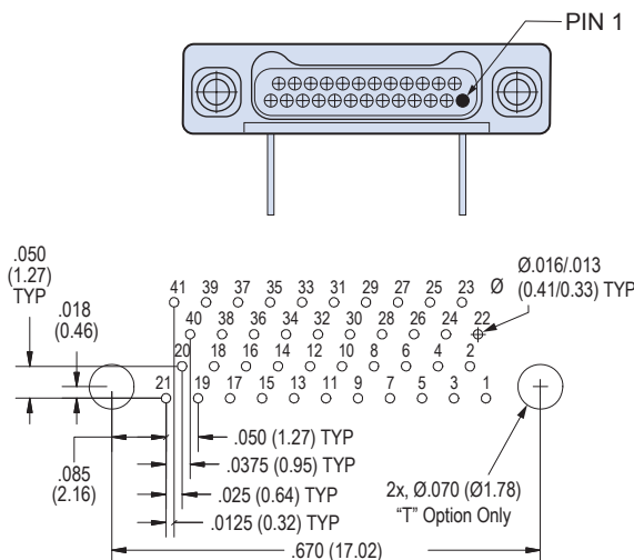
41 Contacts
