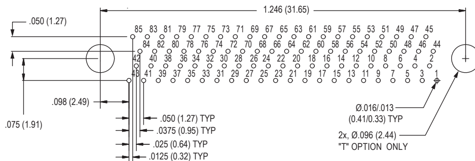
85 Contacts
